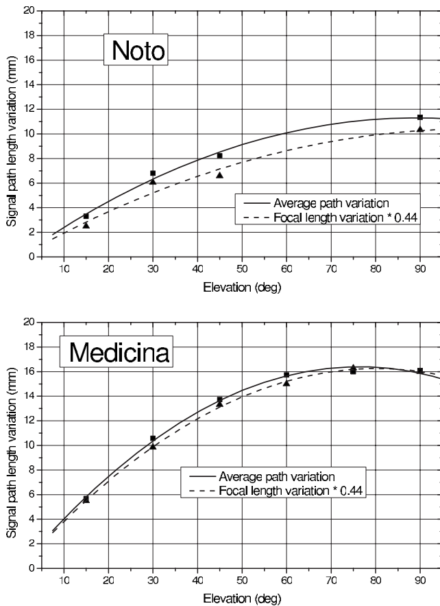
Fig. 12. Contribution of primary reflector deformations to signal path length variation: the two curves are obtained interpolating the signal path variations at four (six) elevation positions for Noto (Medicina) telescope according to Clark and Thomsen (1988) (triangle, dashed line) and to the direct computation of the signal path (see Fig. 11)
