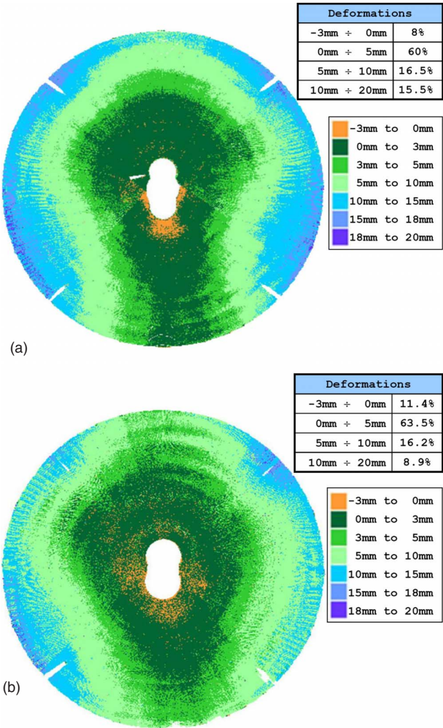
Fig. 8. Relative deformations of the dish between the scanning at 15° and the one at 90° for (a) Medicina; (b) Noto telescopes
