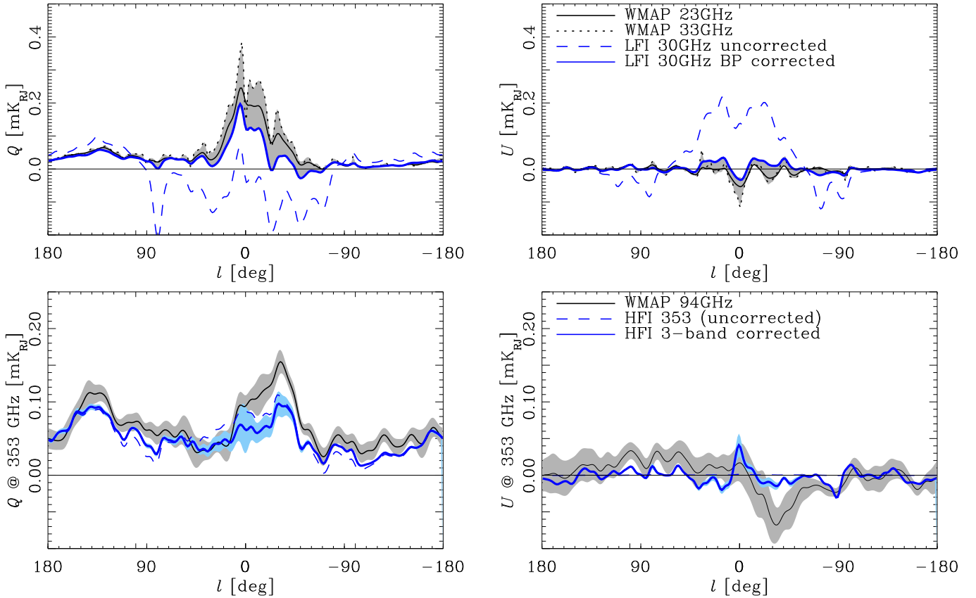
Fig. A.1. Top: comparison of LFI 30 GHz Stokes Q (left) and U (right) with WMAP 23 and 33 GHz along the Galactic plane smoothed to a full width half maximum (FWHM) of 6°. All frequencies are over-plotted by extrapolating the WMAP data to 30 GHz using a synchrotron \beta = -2.95 (Jaffe et al. 2011). The grey band shows the rms variation among them. Bottom: average profile of three HFI frequencies with ground-based bandpass leakage correction. The 143 and 217 GHz frequencies are extrapolated to 353 GHz using the Planck dust model spectrum of Planck Collaboration XI (2014). The dark blue curve shows the average of the frequencies with a pale blue band showing the variance. The WMAP 94 GHz data are also extrapolated to 353 GHz in order to compare its profile in solid black with the grey band showing its variation among different years.
