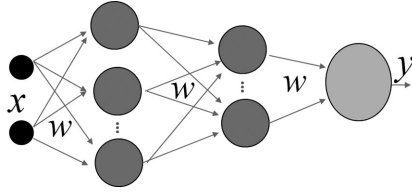
Figure 1. The typical topology of a feed-forward neural network, in this case representing the architecture of MLPQNA. In the example, there are two hidden layers between the input (X) and output (Y) layers, corresponding to the architecture mostly used in the case of complex problems.
