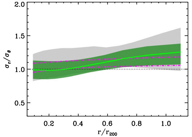
Fig. 8. Velocity anisotropy profile (\sigma_r/\sigma_\theta)(r) for all galaxies of the ensemble cluster (pale green line and shading). Dark green shading: 1\sigma confidence level. Dot-dashed magenta lines: 1\sigma intervals of the \mathcal{L} -weighted average of the 35 MAMPOSSt best-fit model (\sigma_r/\sigma_\theta)(r) . Gray shading: 1\sigma intervals of the result of B+16 for the GCLASS sample.
