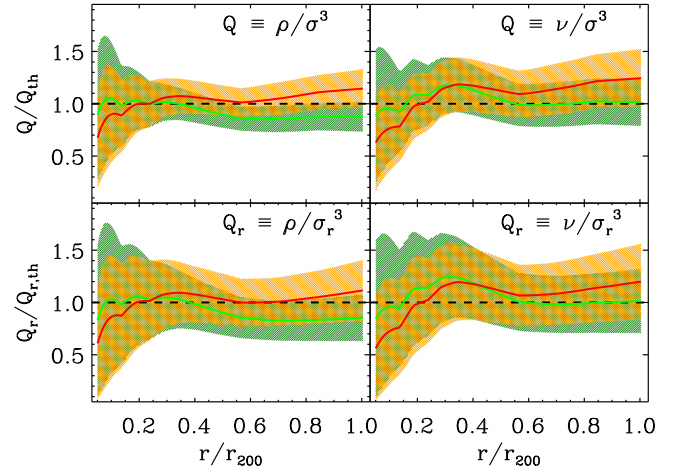
Fig. 10. The pseudo phases-space density profiles of the ensemble cluster. The solid lines show Q(r) and Q_r(r) of the ensemble cluster ( top and bottom panels, respectively) derived from the total mass density profile \rho(r) and the number density profile \nu(r) (left and right panels, respectively), divided by power laws of the radius Q_{th} \propto r^{-1.84} and Q_{r,th} \propto r^{-1.92} (green line and shadings) or by power laws Q_{th} \propto r^{-2.02} and Q_{r,th} \propto r^{-2.11} (red line and orange shading). The shadings indicate 1\sigma uncertainties. The dashed black line is unity.
