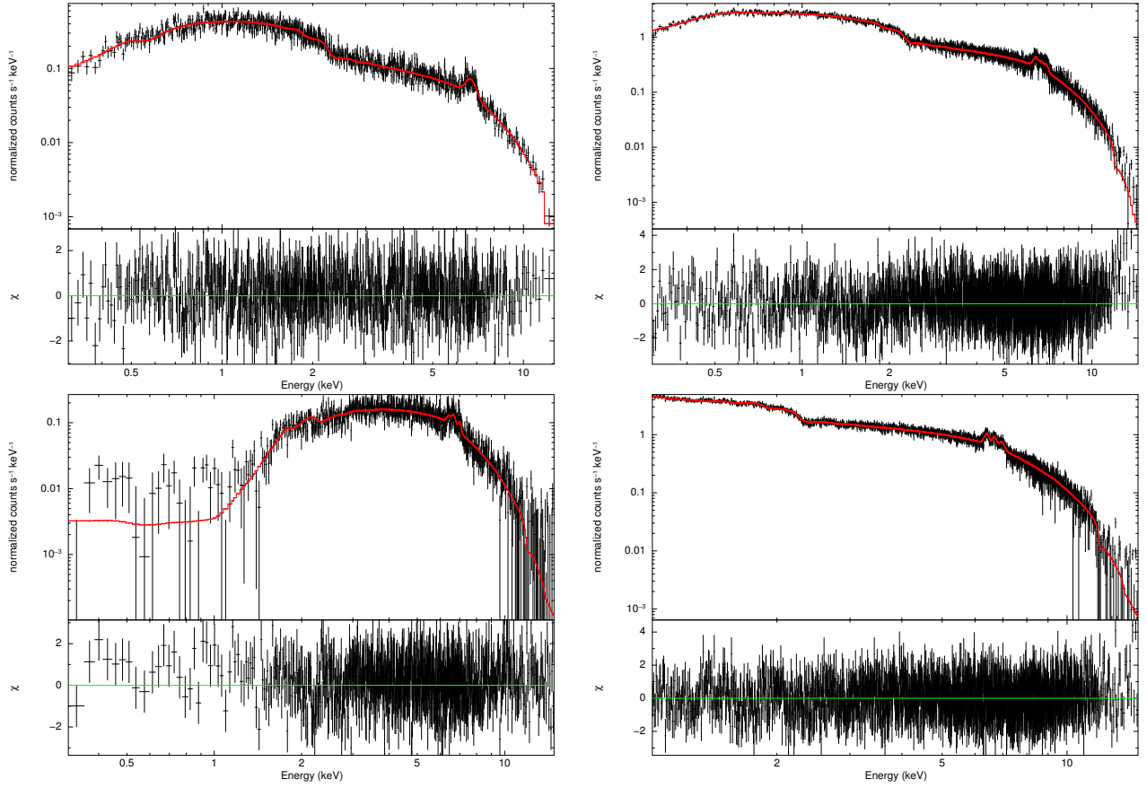
Figure 3. XMM-Newton EPIC pn spectra (in black) and the best fit total model (solid red line). Left top panel: spectrum of IGR J00234+6141 in the 0.3 – 15.0 keV energy range, and the best fit total model TBABS*[COMPTT+GAUSSIAN]. Right top panel: spectrum of IGR 17195-4100 in the 0.3 – 15.0 keV energy range, and the best fit total model TBABS*[COMPTT+(4)GAUSSIAN COMPONENTS]. Left lower panel: spectrum of XY Ari in the 0.3 – 15.0 keV energy range, and the best fit total model TBABS*[COMPTT+(3)GAUSSIAN COMPONENTS]. Right lower panel: spectrum of V1223 Sgr in the 1.0 – 15.0 keV energy range, and the best fit total model TBABS*[COMPTT+(3)GAUSSIAN COMPONENTS]. See Table 2, 3, and 4.
