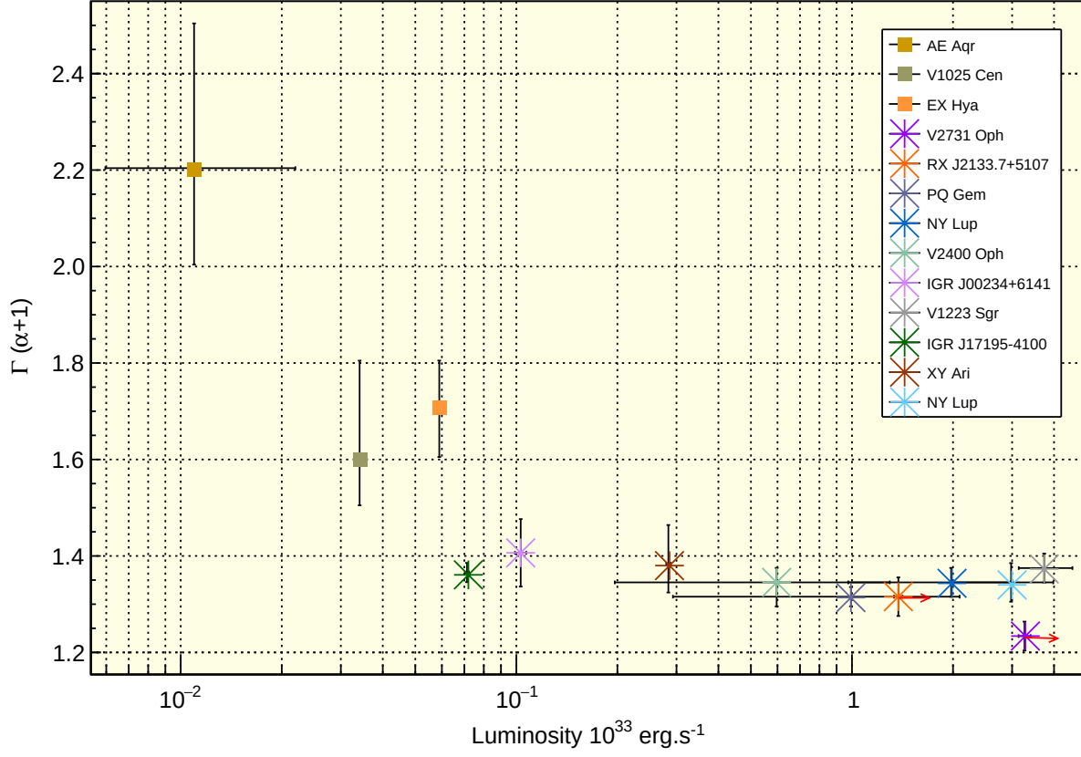
Figure 5. Photon index \Gamma versus luminosity of the unabsorbed Comptonization (COMP TT) component in the ( \sim 0.3 to 15 keV) energy band (see Table 2 and 5). Red arrow indicates lower limit on the luminosity.
