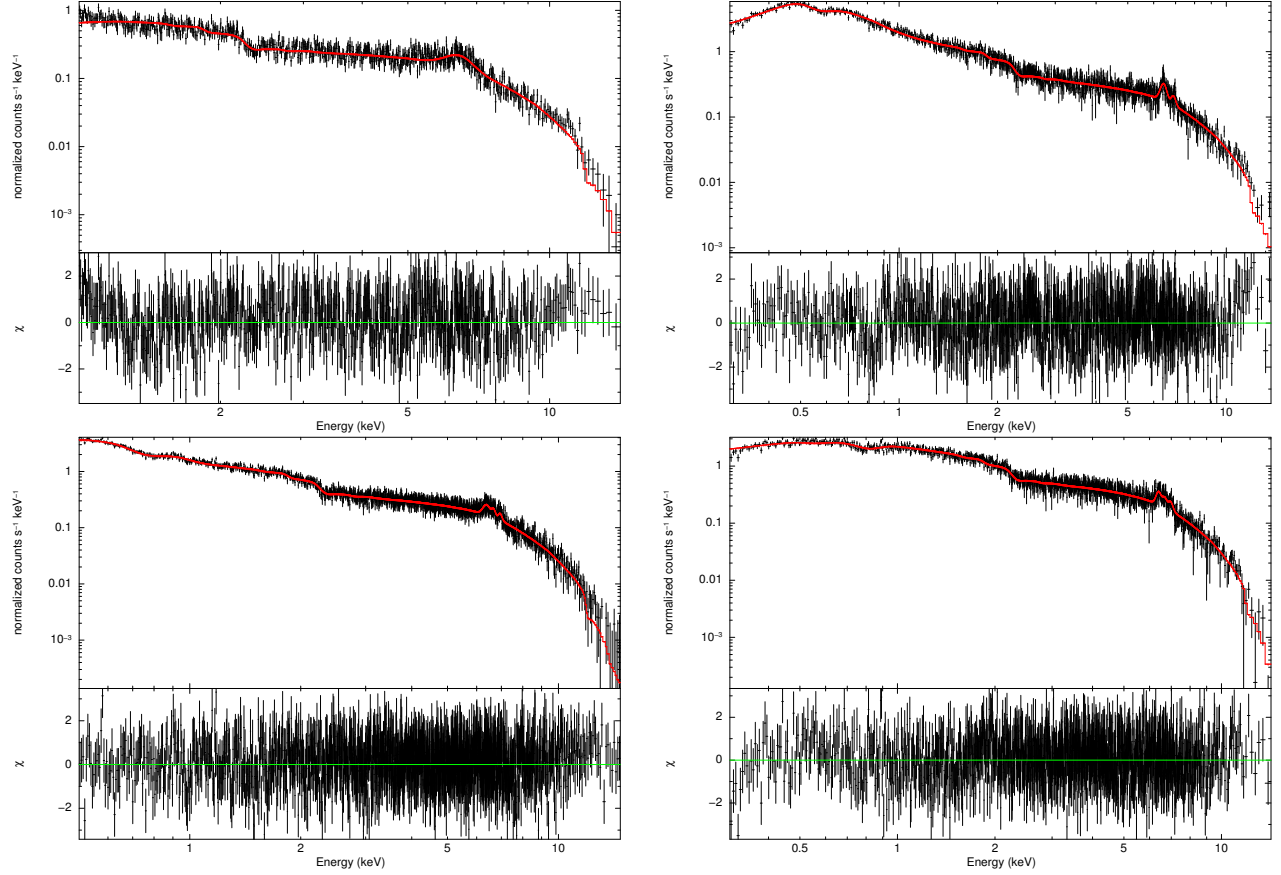
Figure 2. XMM-Newton EPIC pn spectra (in black) and the best fit total model (solid red line). Left top panel: spectrum of V2731 Oph in the 1.0 – 15.0 keV energy range, and the best fit total model TBABS*[COMPTT+GAUSSIAN]. Right top panel: spectrum of RX J2133.7+5107 in the 0.3 – 15.0 keV energy range, and the best fit total model TBABS*[COMPTT+(2)GAUSSIAN COMPONENTS]. Left lower panel: spectrum of PQ Gem in the 0.5 – 15.0 keV energy range, and the best fit total model TBABS*[COMPTT+(5)GAUSSIAN COMPONENTS]. Right lower panel: spectrum of V2400 Oph in the 0.3 – 15.0 keV energy range, and the best fit total model TBABS*[COMPTT+(4)GAUSSIAN COMPONENTS]. See Table 2, 3, and 4.
