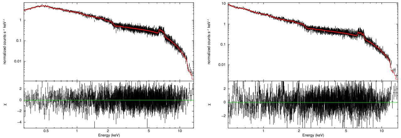
Figure 4. XMM-Newton EPIC pn spectra (in black) and the best fit total model (solid red line). Left panel: spectrum of Obs. ID 0105460301 in the 0.3 – 15.0 keV energy range, and the best fit total model TBABS*[COMPTT+(4)GAUSSIAN COMPONENTS]. Right panel: spectrum of Obs. ID 0105460501 in the 0.5 – 15.0 keV energy range, and the best fit total model TBABS*[COMPTT+(4)GAUSSIAN COMPONENTS]. Table 2, 3, and 4.
