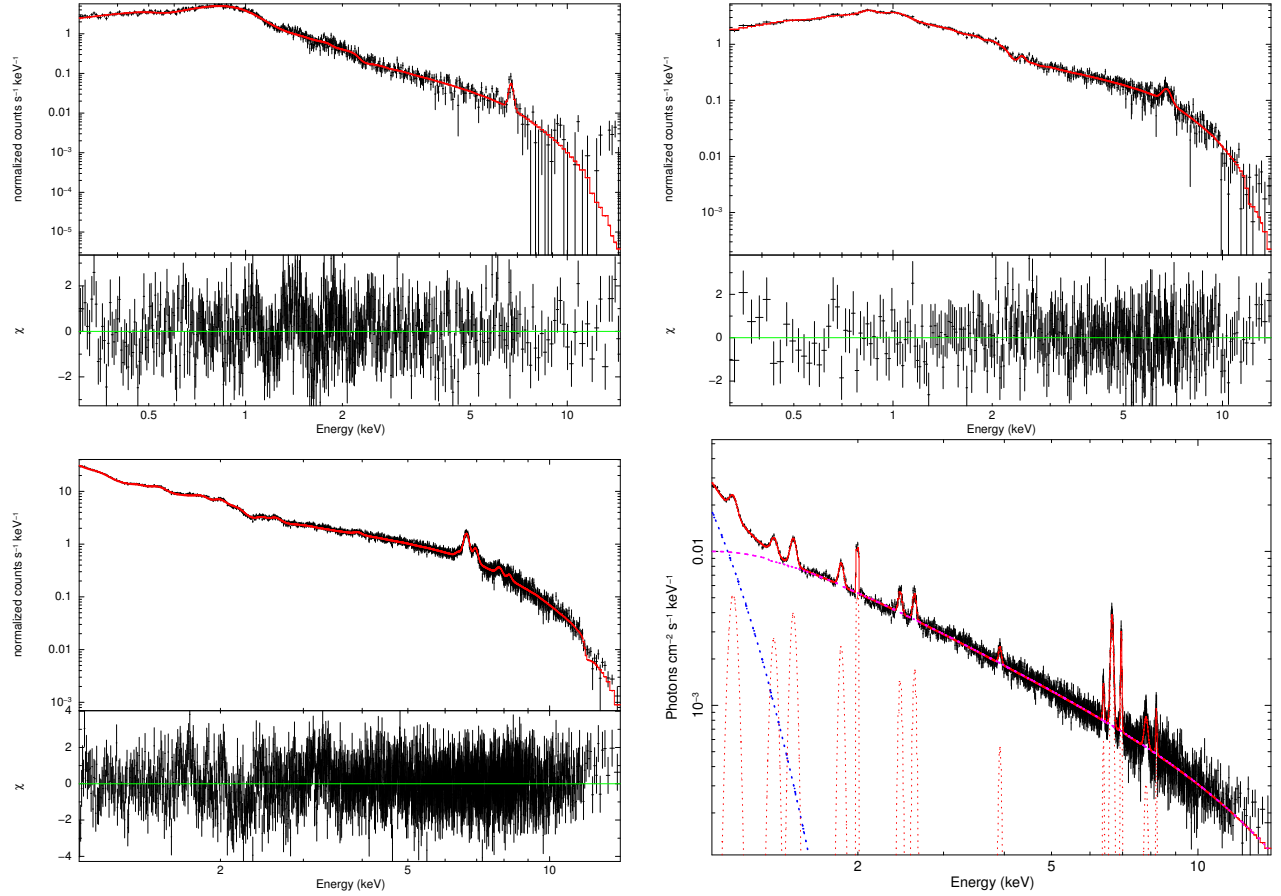
Figure 1. XMM-Newton EPIC pn spectra (in black) and the best fit total model (solid red line). Left top panel: spectrum of AE Aqr in the 0.3 – 15.0 keV energy range, and the best fit total model TBABS*[COMPTT+(2)GAUSSIAN COMPONENTS]. Right top panel: spectrum of V1025 in the 0.3 – 15.0 keV energy range, and the best fit total model TBABS*[COMPTT+(5)GAUSSIAN COMPONENTS]. Left lower panel: spectrum of EX Hya in the 1.0 – 15.0 keV energy range, and the best fit total model TBABS*[COMPTT+(13)GAUSSIAN COMPONENTS]. Right lower panel: unfolded spectrum of EX Hya in the 1.0 – 15.0 keV energy range; the total model in red, the BBODY component in blue, the COMPTT component in magenta, and the GAUSSIAN components in dashed red lines. See Table 2, 3, and 4.
