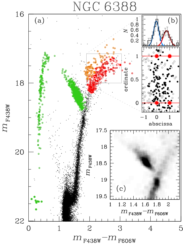
Figure 8. Overview of NGC 6388 features. Panel (a) shows the m_{F438W} versus m_{F438W} - m_{F606W} CMD: HB, RGB, and AGB stars are highlighted in green, red, and orange, respectively. Panels (b) shows the verticalized RGB sequence using the stars of the grey box of panel (a); the ‘abscissa’ distribution of the verticalized sequence is shown in the upper panel. A bi-Gaussian function is fitted to the abscissa distribution. Panel (c) illustrates the Hess diagram around the CMD region containing the red clump and the RGB bump.
