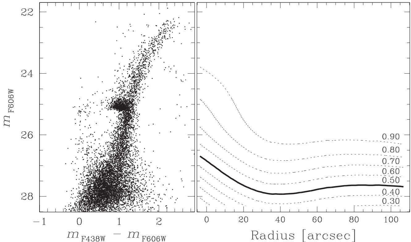
Figure 3. Left-hand panel shows the m_{F606W} versus m_{F438W} - m_{F606W} CMD of all the well-measured stars in the field of view containing G1. Right-hand panel shows the completeness levels of our catalogue as a function of the F606W magnitude and of the radial distance from the centre of the cluster.
