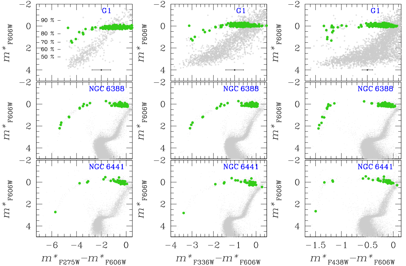
Figure 9. Transformed m_{F606W}^* versus m_X^* - m_{F606W}^* CMDs, with X = F275W, F336W, and F438W , for the HB stars of G1 (first row), NGC 6388 (second row), NGC 6441 (third row), respectively. The left-hand panels are the m_{F606W}^* versus m_{F275W}^* - m_{F606W}^* CMDs, the middle panels are the m_{F606W}^* versus m_{F336W}^* - m_{F606W}^* CMDs, while the right-hand panels show the m_{F606W}^* versus m_{F438W}^* - m_{F606W}^* CMDs of the GCs listed above. The green points are the HB stars located between 2.5 \times r_h and 4.5 \times r_h from the cluster centres. Top left panel reports the completeness of G1 catalogue at different magnitude levels.
