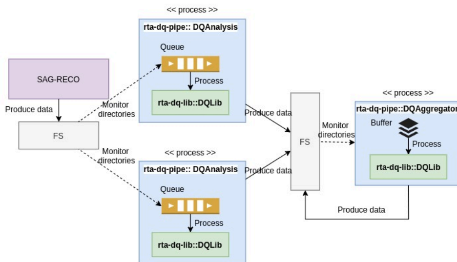
Figure 23: SAG-DQ process view
