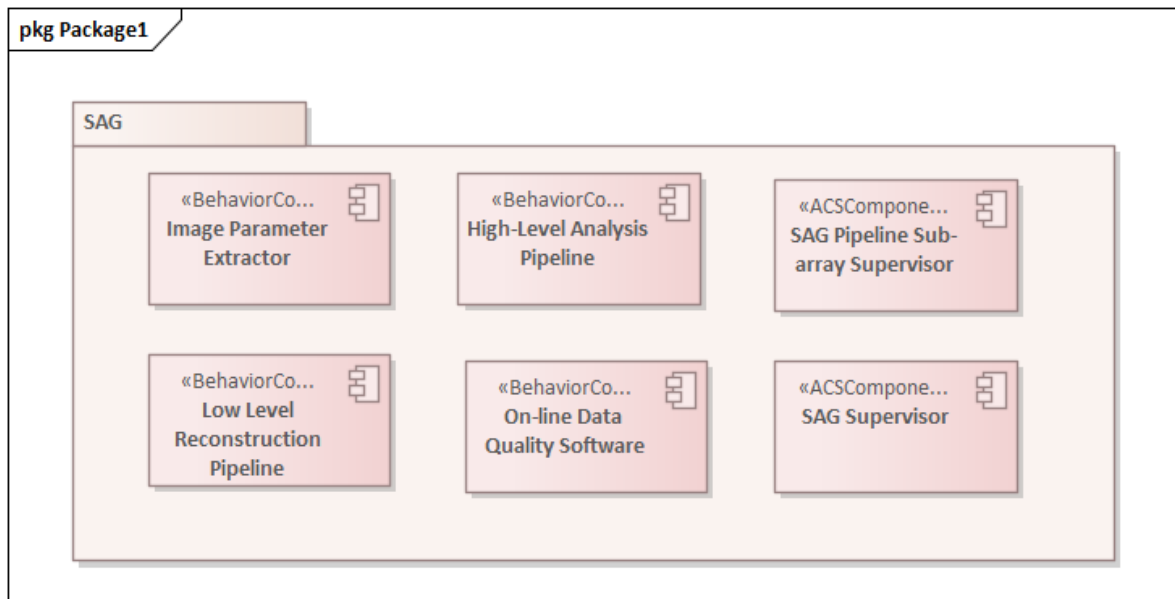
Figure 3: Package diagram illustrating the internal structure of the SAG sub-system.
