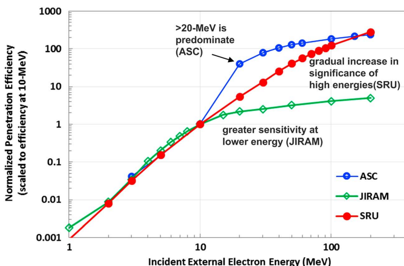
Figure 2. Comparison of spectral sensitivities of the ASC, SRU, and JIRAM. Probabilities for omnidirectional high-energy electrons to penetrate instrument shielding and create image noise events (“penetration efficiencies”) have been normalized to the value at 10 MeV for each instrument.
