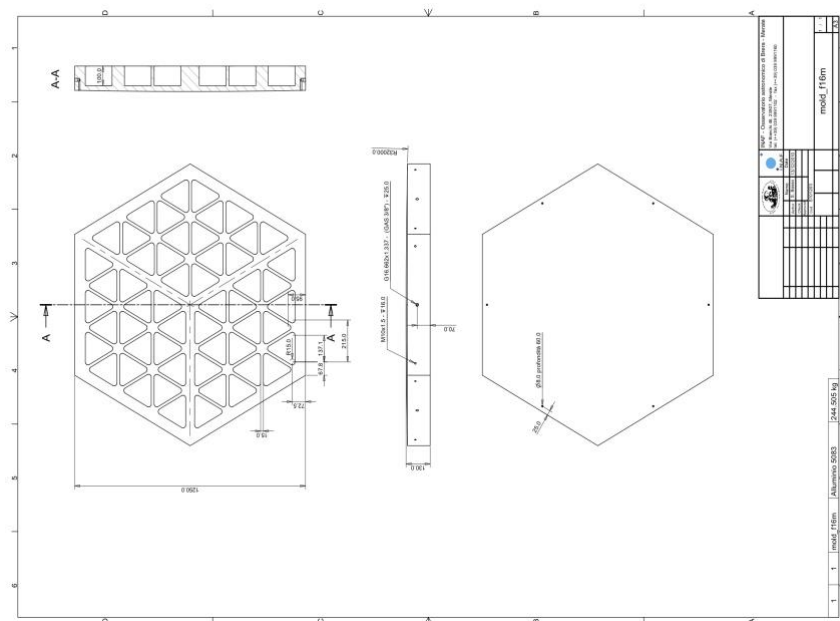
Figure 2: Mould design.
