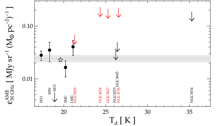
Fig. 4. \epsilon_{30\text{GHz}}^{\text{AME}} vs T_d . Red symbols are for SRT targets. The shaded area shows the weighted average and standard deviation of \epsilon_{30\text{GHz}}^{\text{AME}} ; the star is the PLA16 estimate for the MW (see text for details).
