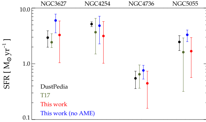
Fig. 3. Comparison between SFRs from DustPedia and from S_{5\text{GHz}}^{\text{ff}} (see text for details).
