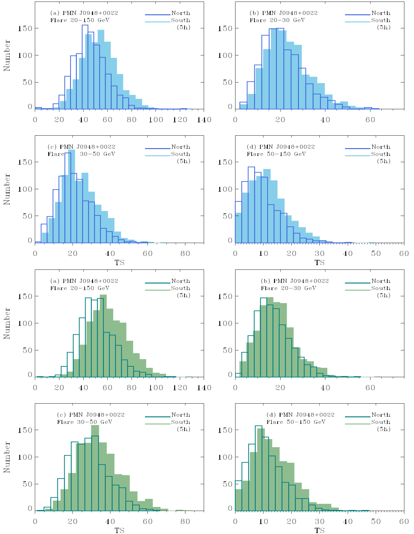
Figure A1. PMN J0948+0022 in ‘flare’ (exposure 5h): comparison of distributions of the TS values depending on the energy band for detection. Blue: edisp=no, green: edisp=yes. See Table 3 and A1 for details.
