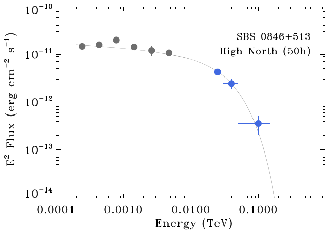
Figure 2. Spectral energy distribution (SED) of SBS 0846+513 in the high state. The grey line is the input model; the blue points are the simulated fluxes for 50 h of exposure. The grey points are from Paliya et al. (2016; F2 flare).
