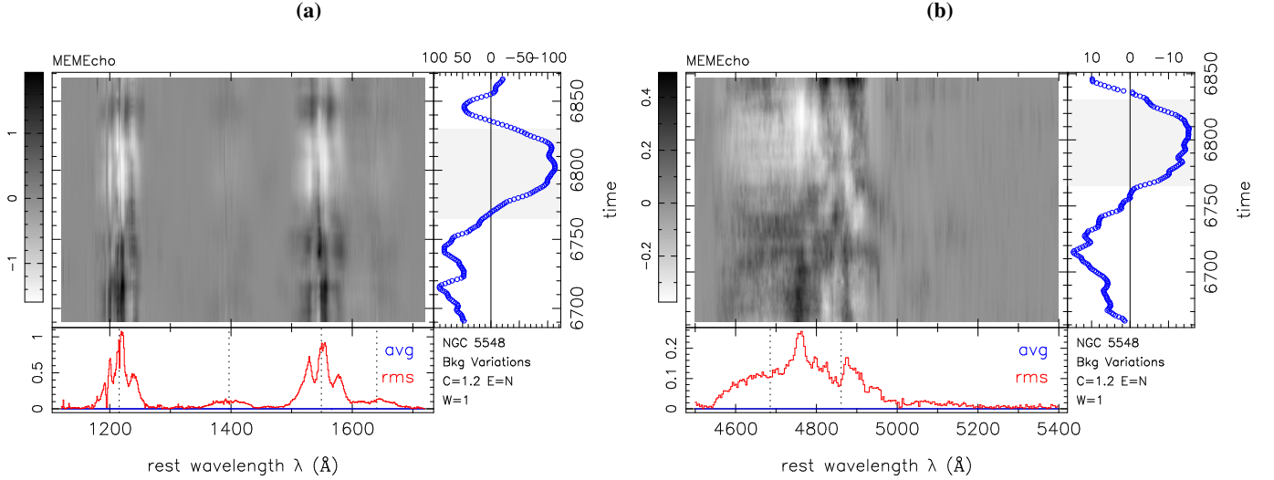
Figure 10. The slowly-varying background component L_0(\lambda, t) of the MEMECHO model fitted to the HST data (left) and MDM data (right). The model’s time-averaged spectrum has been subtracted to leave time-varying residuals. The right panels show the wavelength-averaged response, with gray shading indicating the BLR Holiday dates. The lower panels show the mean (blue) and rms (red) of the time-dependent residuals at each wavelength. All lines show a depressed flux during the BLR Holiday. The helical Barber-Pole pattern, with stripes moving from red to blue across the line profile, is evident in the C IV and Ly \alpha residuals. The Barber-Pole pattern is absent in He II and may be present in H \beta but with a less clear pattern.
