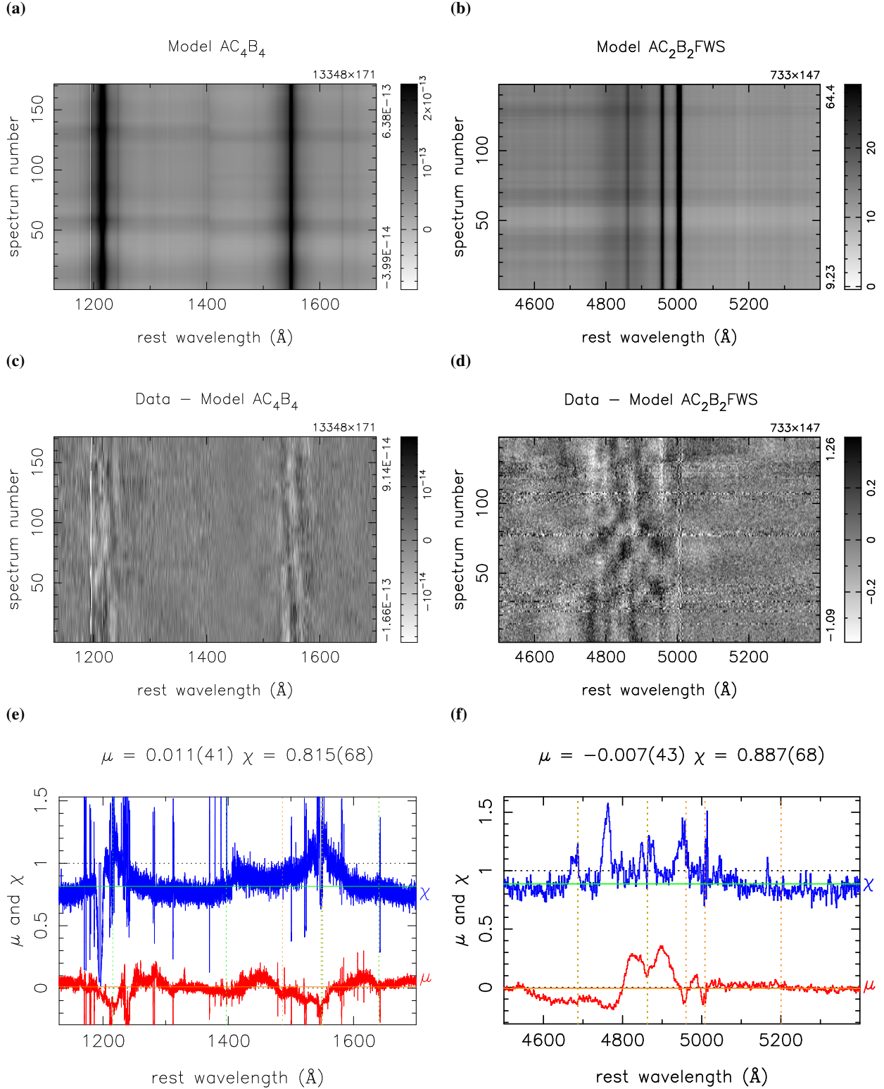
Figure 3. Model (a,b) and residuals (c,d) of the PREPSPEC fit to the HST (left) and MDM (right) data. Lower panel shows the mean (red) and rms (blue) over time of the normalized residuals for HST (e) and MDM (f). Note in panel (c) the helical “Barber-Pole” pattern of stripes moving from red to blue across the C IV and Ly \alpha line profiles. The Model specification key includes components A=average spectrum, C_n =continuum polynomial with n parameters, B_n =BLR for n emission lines, and for the MDM data the calibration adjustments F=flux, W=wavelength and S=seeing.
