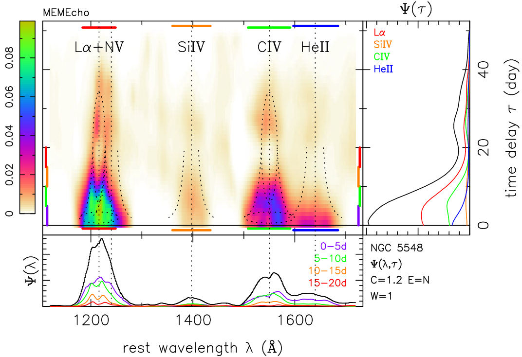
Figure 6. As in Fig. 5, showing the two-dimensional wavelength–delay map \Psi(\lambda, \tau) reconstructed from the MEMECHO fit to the UV spectra from HST . The ellipses shown for Ly \alpha and C IV correspond to Keplerian disk orbits at R = 2 and 20 light days.
