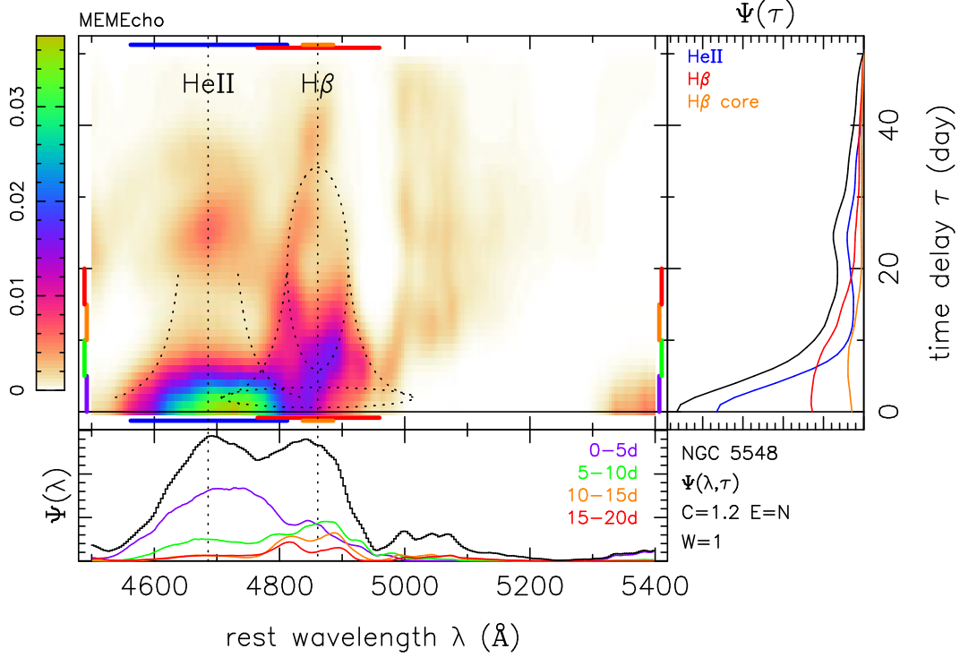
Figure 5. Two-dimensional wavelength–delay map \Psi(\lambda, \tau) reconstructed from the MEMECHO fit to the optical spectra from MDM. Delays are measured relative to the 1150 Å continuum light curve. Panels below and to the right of the map give the projected responses \Psi(\lambda) and \Psi(\tau) . Here the black curve is the full response and the colored curves are for the wavelength or delay ranges indicated by the correspondingly colored bars in the margins of the map. Dotted curves show the envelope around each line inside which emission can occur from a Keplerian disk inclined by i = 45^\circ orbiting a black hole of mass M_{\text{BH}} = 7 \times 10^7 M_\odot . The ellipses shown for H \beta correspond to Keplerian disk orbits at R = 2 and 20 light days.
