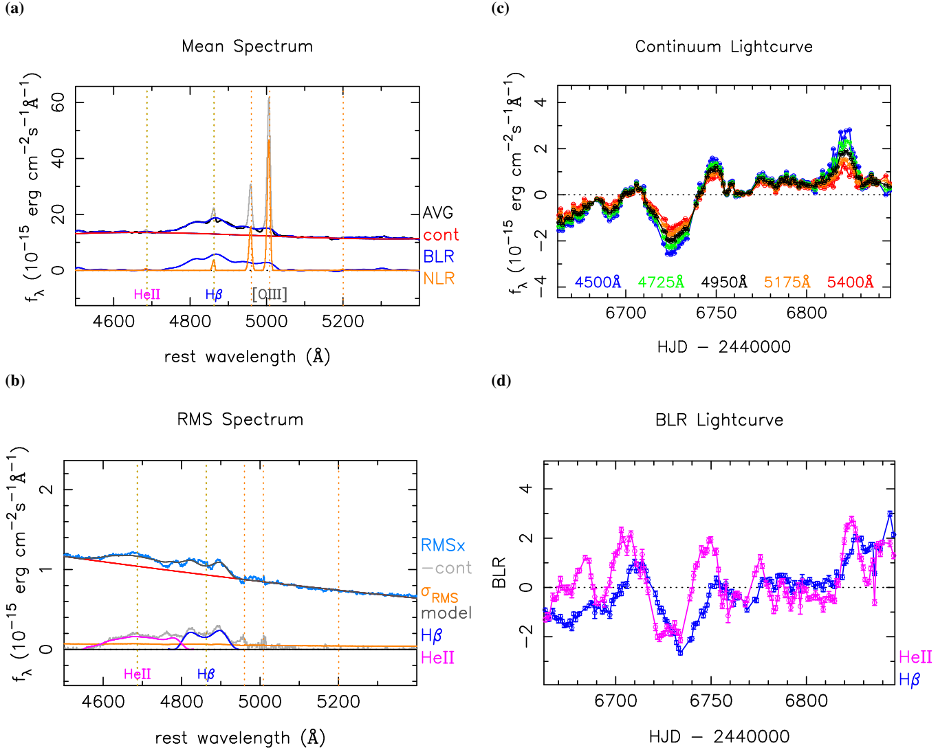
Figure 2. As in Fig. 1 but here showing results of the PREPSPEC fit to the MDM data covering the optical spectral region including the broad H \beta and He II \lambda 4686 and narrow [O III] emission lines.
