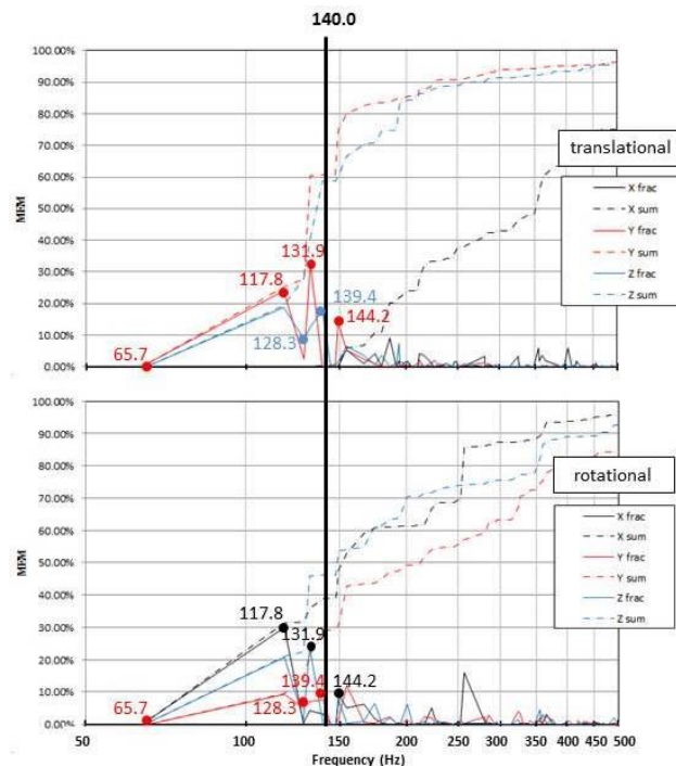
Figure 27. Normal mode analysis result : modal effective mass (MEM) as a function of frequency. Six first eigenfrequencies are indicated with dots. Continuous line is fractional MEM, dotted line is summed MEM. Top: translational degrees of freedom. Bottom: rotational degrees of freedom.
