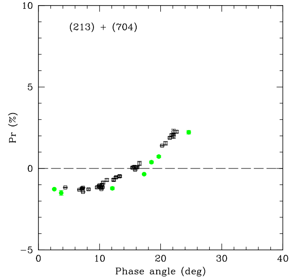
Figure 7. Available phase-polarization measurements in V colour for the two F-class asteroids (213) Lilaea (green symbols) and (704) Interamnia (black symbols). There are differences between the two objects, but both exhibit an inversion angle of polarization, between about 16^\circ and 18^\circ , which is low in comparison to the vast majority of asteroids belonging to other taxonomic classes.
