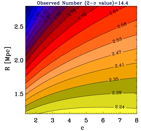
Fig. 3. 2-σ limits on the thermal relic mass m_{\chi} (coloured contours) are shown for different assumed values of the concentration parameter c (horizontal axis) and for the cluster radius R (vertical axis)
