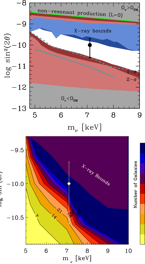
Fig. 5. Top panel: constraints on the sterile neutrino parameter space from Eq. (3). The allowed region is the white area. Taking the abundance \phi_{\text{obs}} corresponding to our observed number of galaxies in the target field within 1\text{-}\sigma and 2\text{-}\sigma confidence levels ( \phi_{\text{obs}} = 19.3 and \phi_{\text{obs}} = 14.4 , respectively) yields the exclusion regions shown as red shaded areas. Our constraints are compared with upper bounds from X-ray observations of the Milky Way and dwarf galaxies (as reported in Riemer-Sørensen 2014). Grey areas are excluded by current limits on the abundance of DM (Ade et al. 2015). The green line corresponds to the non-resonant DW case with vanishing lepton asymmetry L = 0 . We also show the constraints obtained from the abundance of satellites in the Milky Way by Schneider (2016, dashed line) and by Lovell et al. (2016, solid line). The tentative line signal at 3.5 keV corresponding to a sterile neutrino mass m_\nu = 7.1 keV (Bulbul et al. 2014; Boyarsky et al. 2014) is shown by the point with errorbars. Bottom panel: the coloured contours correspond to the different values of \phi_{\text{field}} corresponding to a given combination of \sin^2(2\theta) - m_\nu . In both panels we assumed c = 3 and R = 1.6 Mpc as reference values. The sensitivity of the curves to changes in such parameters is the same as the thermal WDM case, shown in Fig. 3.
