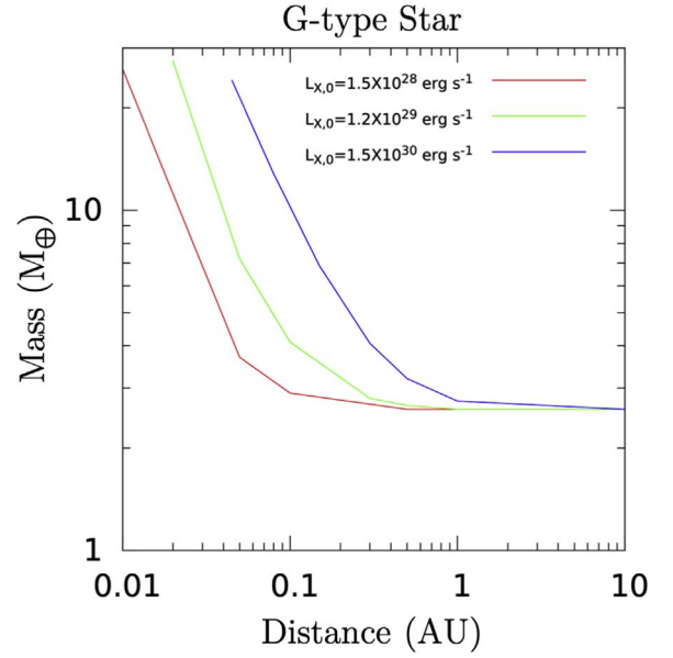
Figure 8. Mass threshold functions calculated using the model from Locci et al. (2019) for G-type stars for different initial X-ray luminosities (Penz et al. 2008). The UV luminosities scale with the X-ray ones according to the models by Sanz-Forcada et al. (2011).
