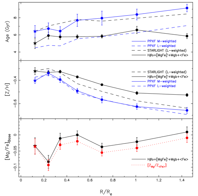
Figure 8. Age, Z , and [Mg/Fe] profiles as a function of galactocentric radius obtained from different methods by using STARLIGHT , PPXF, and index fitting. Results from STARLIGHT and PPXF are presented as black and blue lines, respectively, index fitting is indicated by filled black circles, and the [Z_{Mg}/Z_{Fe}]_{\text{Base}} values are shown by the red line. The filled star in each panel indicates the NSC-contaminated bin.
