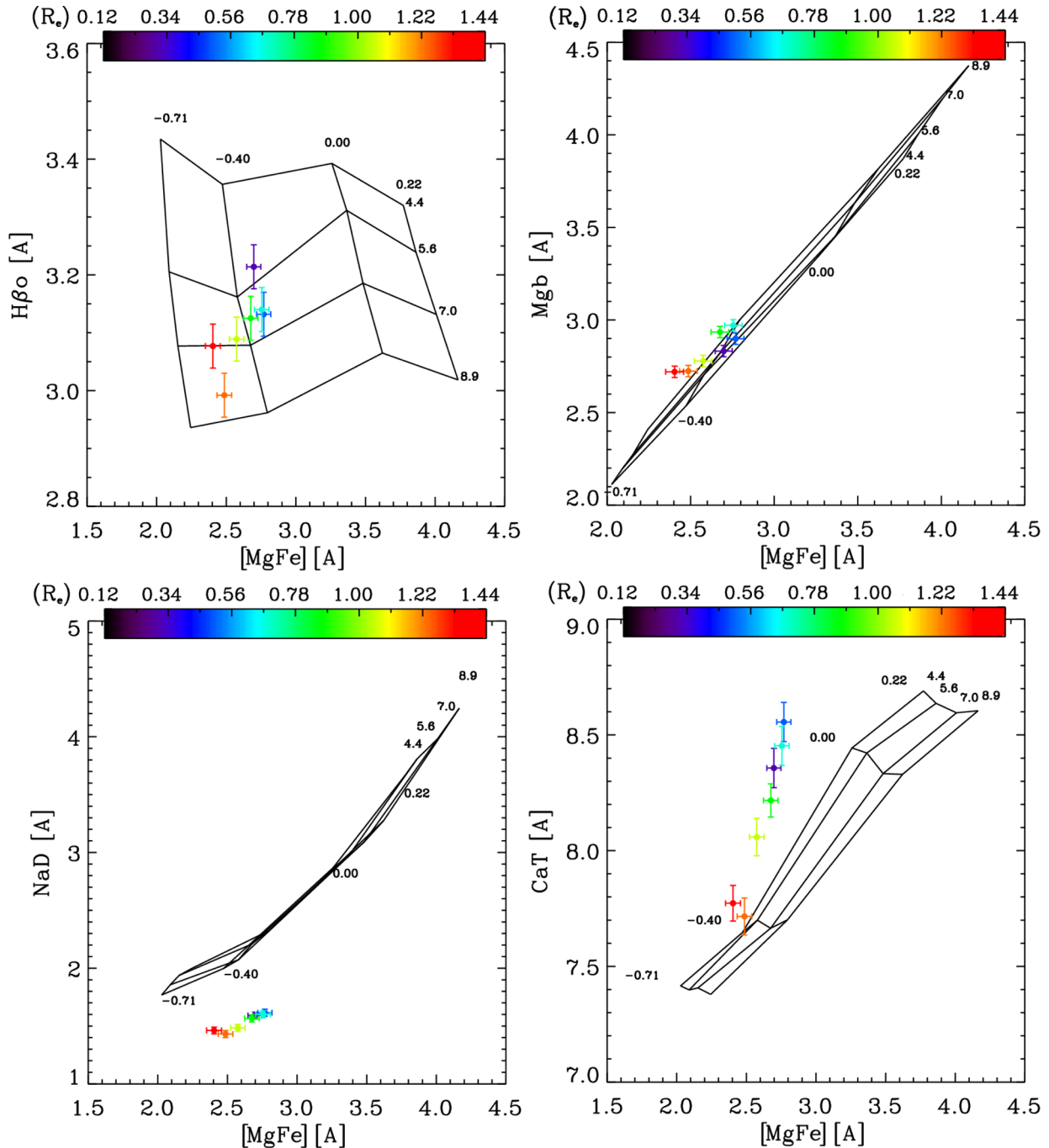
Figure 12. Index–index diagrams of H\beta_o , \text{Mgb} , \text{NaD} , and \text{CaT} as function of total metallicity [\text{MgFe}] . MIUSCAT models grids are plotted with IMF slope of 1.3, age ranging between 4.4 and 8.9 Gyr and metallicity ranging between -0.71 and 0.22 dex. The colour coding indicates the radial distance in R/R_e , where red indicates the most distant radial bin from the centre.
