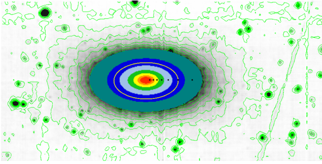
Figure 6. Contour map of NGC 1396 with radial bins overlaid on NGC 1396, with luminosity-weighted bin centres indicated with black dots. The effective radius ( R_e=10.7 arcsec) is indicated with a yellow ellipse.
