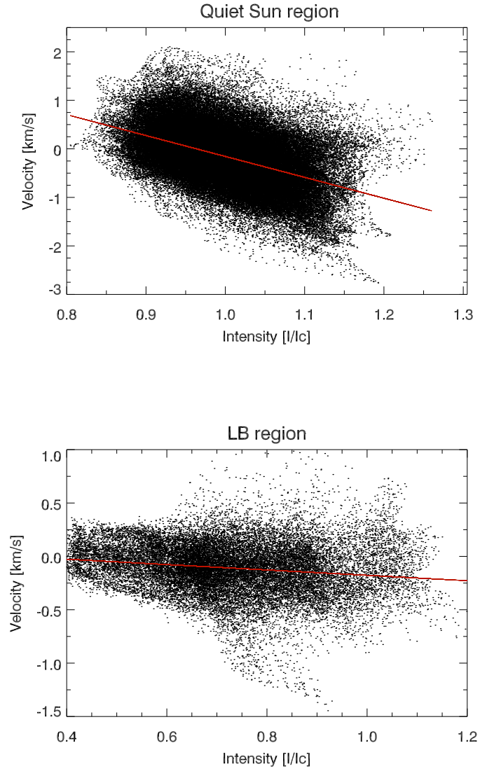
Figure 10. Scatter plots of intensity and LOS velocity in a region of the quiet Sun (top panel) and in the region of the LB (bottom panel). The data plotted in the latter plot include values of the five sequences studied in Figure 5. The red line in each plot represents the linear fit of the dataset analysed.
