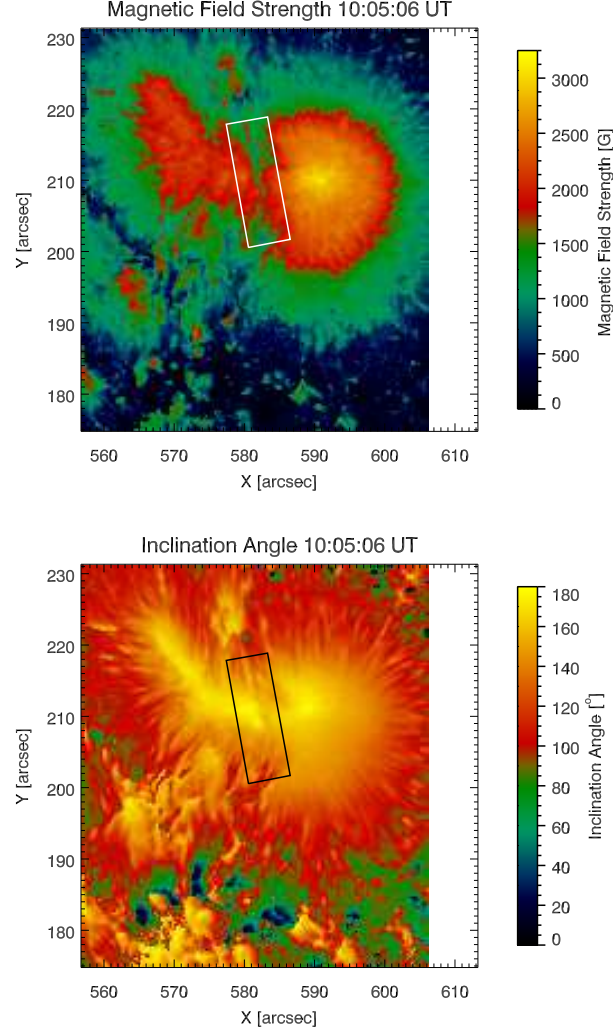
Figure 4. Maps of the magnetic field strength and inclination angle in the local solar frame coordinate obtained from the inversion of both the Fe I 630.15 nm and 630.25 nm line datasets taken by Hinode on 6 August 2011 at 10:05:06 UT. The region with X > 606'' is not covered by Hinode observations. In the bottom panel 0^\circ and 180^\circ correspond to the directions of radially outward and inward magnetic field, respectively. In each map the solid box indicates the LB's FOV analyzed in the text.
