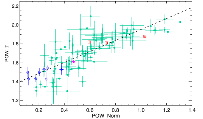
Fig. 7. Relation between the photon index \Gamma and the normalisation of the power-law (pow) continuum as described in Sect. 3.1. The pow normalisation is shown in units of 10^{52} photons \text{s}^{-1} \text{keV}^{-1} at 1 keV. The data in green filled circles represent the Swift data from the obscured epoch (Feb. 2012 onwards), the blue open diamonds are the Swift data from the unobscured epoch of 2005 and 2007, the red open squares represent three XMM-Newton observations from unobscured epoch of 2000 and 2001, and the single filled magenta star corresponds to the stacked data from our summer 2013 campaign when the source was obscured. The data have been fitted with Eq. (3) shown in dashed black line.
