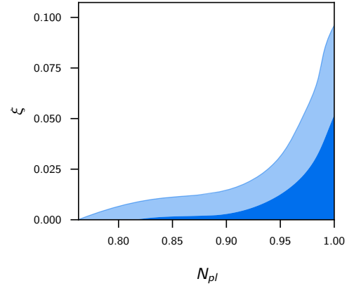
FIG. 18. 2D marginalized confidence levels at 68% and 95% for (N_{\text{pl}}, \xi) for NMC \xi > 0 with Planck TT + lowP + lensing + BAO.
