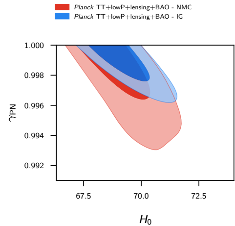
FIG. 24. 2D marginalized confidence levels at 68% and 95% for (H_0, \gamma_{\text{PN}}) for NMC \xi > 0 (red) and IG (blue) with Planck TT + lowP + lensing + BAO.
