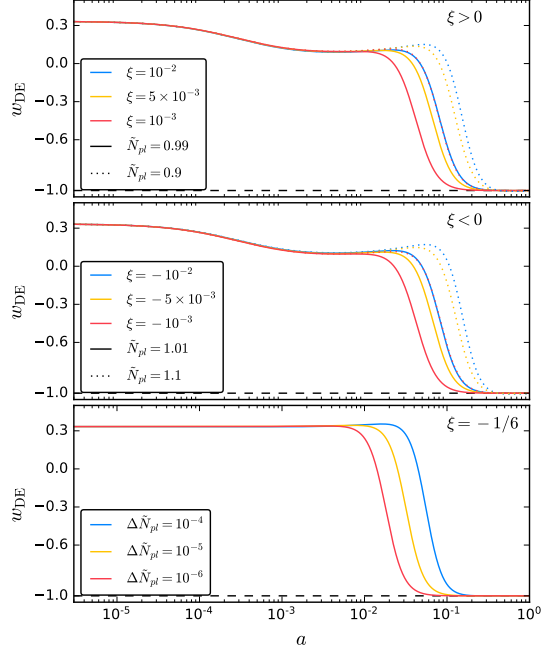
FIG. 2. Evolution of w_{DE} for different values of N_{pl} and \xi . We plot the effective parameter of state for DE for \xi > 0 in the upper panel, \xi < 0 in the central panel, and the CC case \xi = -1/6 in the bottom panel.
