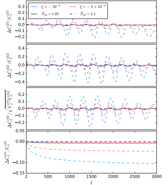
FIG. 13. From top to bottom: relative differences of the TT-EE-TE- \phi\phi power spectra with respect to the \Lambda CDM model for \tilde{N}_{pl} = 1.01, 1.1 and different values of \xi = -10^{-2}, -5 \times 10^{-3} .
