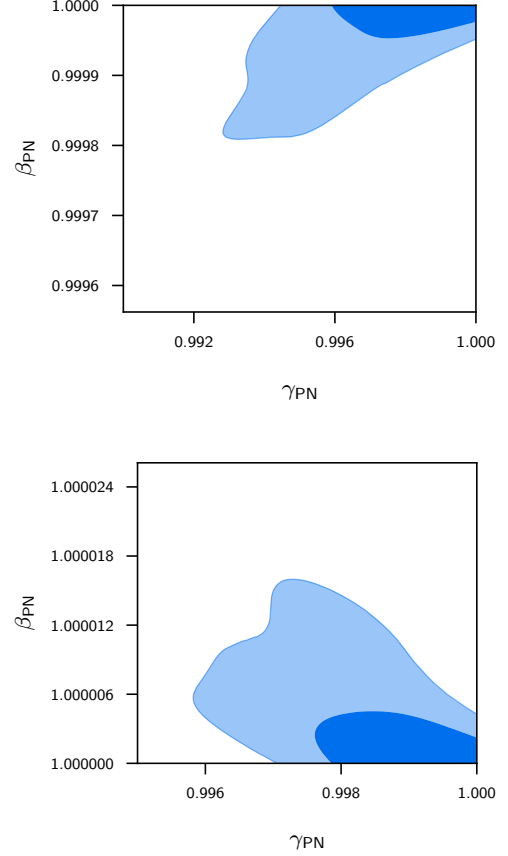
FIG. 23. 2D marginalized confidence levels at 68% and 95% for (\gamma_{\text{PN}}, \beta_{\text{PN}}) for NMC \xi > 0 (left panel) and \xi < 0 (right panel) with Planck TT + lowP + lensing + BAO
