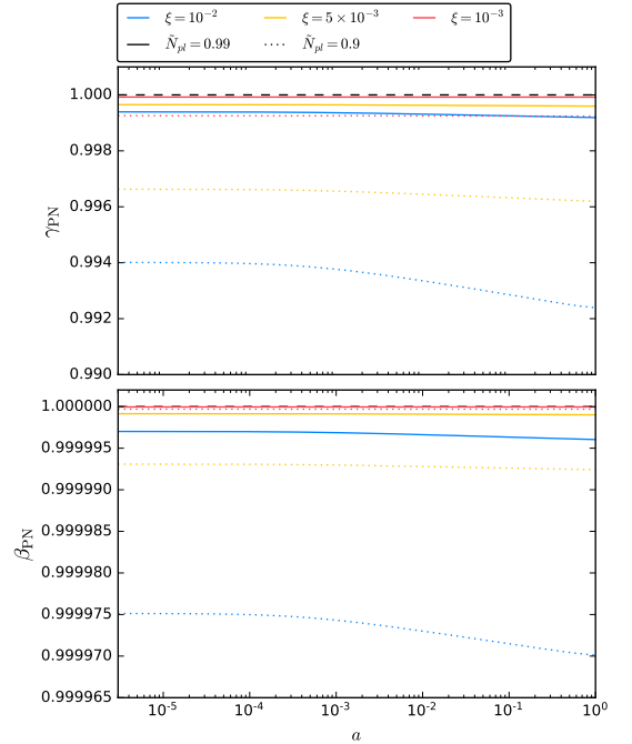
FIG. 7. Evolution of the post-Newtonian parameters \gamma_{\text{PN}} and \beta_{\text{PN}} for different values of N_{pl} and \xi . We show the case with \xi > 0 .
