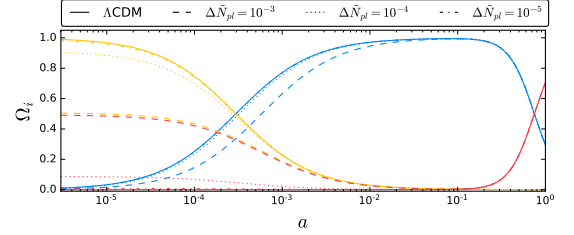
FIG. 5. Evolution of the density parameters \Omega_i : radiation in yellow, matter in blue, and effective DE in red. We plot the CC case \xi = -1/6 for \Delta\tilde{N}_{pl} = 10^{-3} , 10^{-4} , 10^{-5} .
