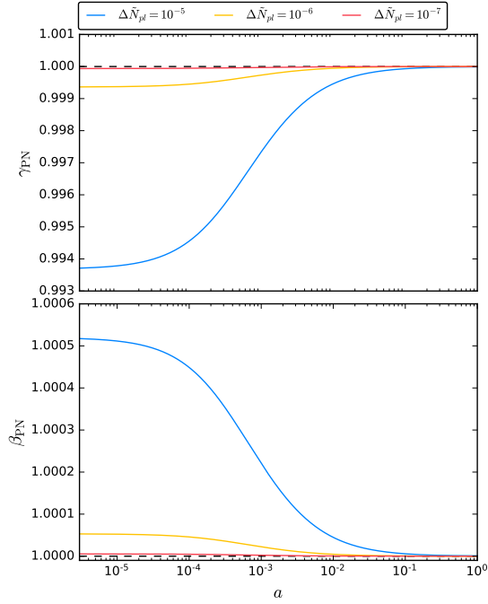
FIG. 9. Evolution of the post-Newtonian parameters \gamma_{\text{PN}} and \beta_{\text{PN}} for different values of N_{\text{pl}} . We show the NMC case \xi = -1/6 , i.e. the CC case.
