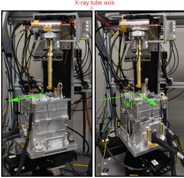
Figure 6: Set-up of the two measurements carried out for decoupling the intrinsic instrumental response to unpolarized radiation from the signal due to the genuine source polarization.
