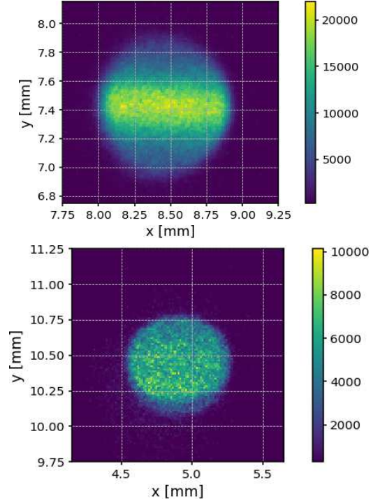
Figure 22: Spot obtained after the alignment of the polarized source at 2.7 keV (top) and 6.4 keV (bottom) with the T-collimator. Images were acquired with ICE test imager, but the source was moved to the same distance as that used for DU calibration.
