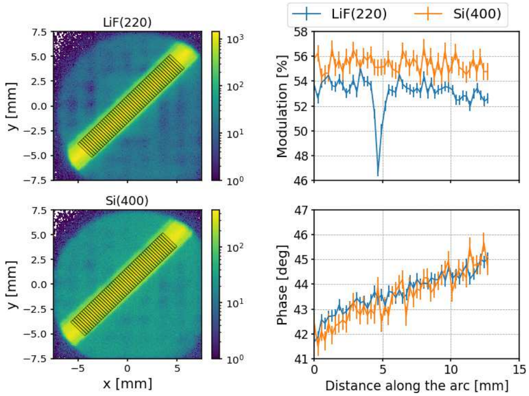
Figure 19: Study of the polarization along the Bragg arc obtained by diffracting 6.4 keV photons generated with an X-ray tube with Fe anode on LiF (220) and Si (400) crystals. The image of the Bragg arc (in the left top and bottom panels) is divided in rectangular regions and for each the modulation and phase measured are reported on the right panels. Modulation of photons diffracted on LiF (220) presents a drop, whose origin is still under investigation. Modulation of Si (400) is on average higher than that of LiF (220) as the Bragg angle is closer to 45 degrees for the first crystal.
