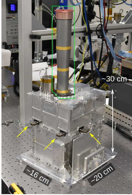
Figure 1: One of the IXPE DU, manufactured in INFN. The stray-light collimator (enclosed in the green box) is removed at the beginning of DU calibration to decrease the distance between the detector and the source (see Section 6.3). Yellow arrows show the three mechanical references of the GPD for alignment.
