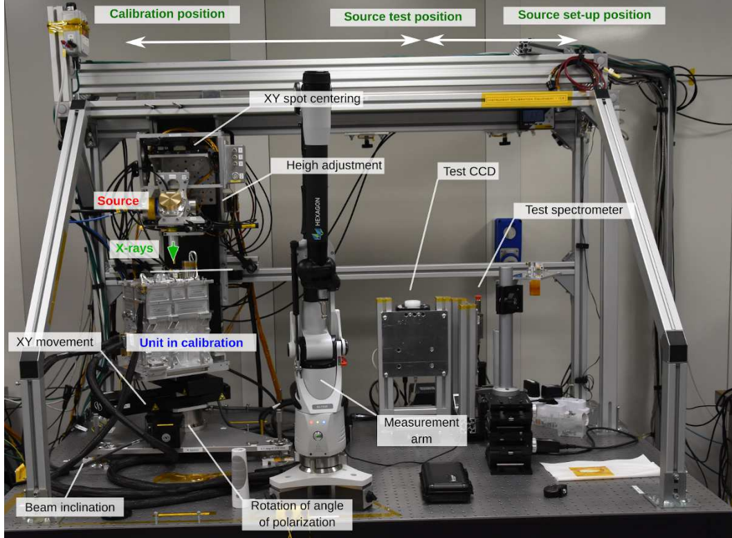
Figure 3: Overview of the ICE. The measurement arm used for alignment, see Section 6.1, is at center. Two commercial detectors (on the right) are available to test the source before the calibration of the DU.
