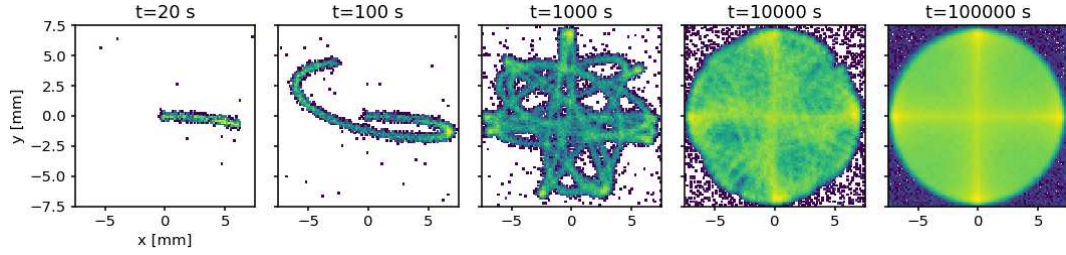
Figure 24: Example of the movement of the polarized source spot due to dithering in case of a flat field illumination.
