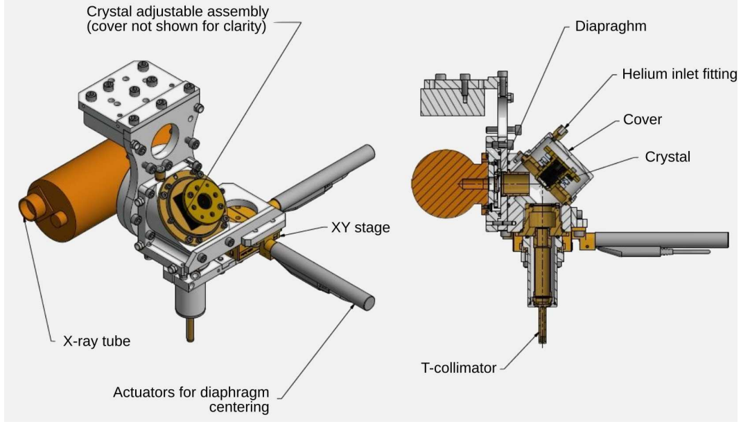
Figure 13: Drawing (top) and cut-view (bottom) of the ICE polarized source.
