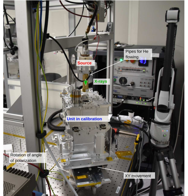
Figure 5: Picture of the ACE with DU-FM2.
