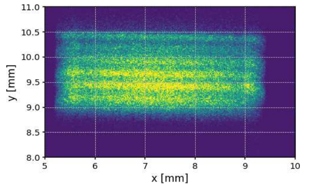
Figure 23: Example of the scan with the T-collimator. The image is acquired with the ICE test imager. This is equivalent to the middle panel of Figure 20. Strips are the tracks of the spot during the scan.
