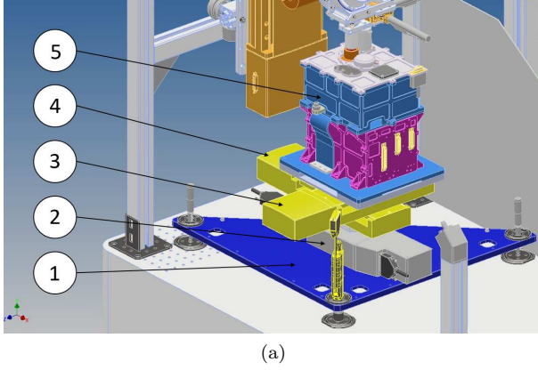
Figure 4: Detailed view of the tower supporting the DU (a) and of the source assembly (b). The items in the figures are the manual and motorized stages which allow one to align the X-ray beam and the DU (item 5). The beam is centered on the detector with two linear stages, item 3 and 4, and its angle of polarization with respect to the detector is changed with a third rotation stage (item 3). The detector tip/tilt is adjusted with a platform (item 1). The source height and tip/tilt are changed with item 6 and 7, respectively, and its position is slide with a manual stage (item 8).
