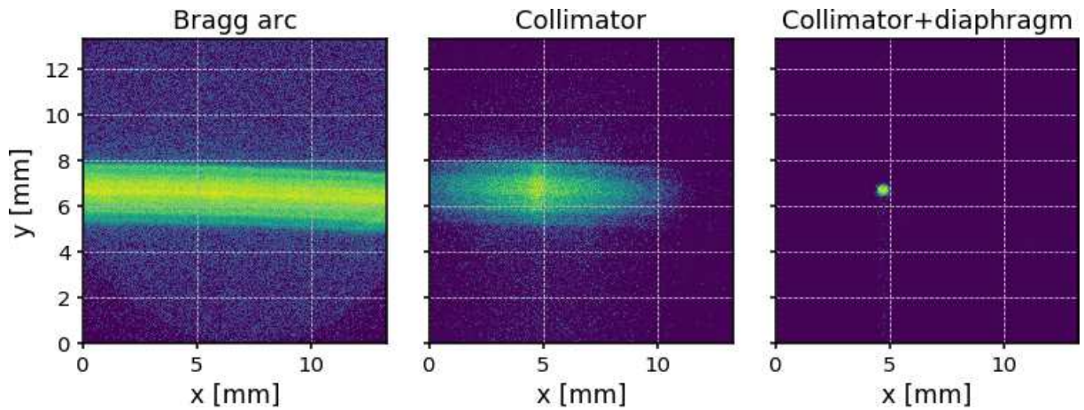
Figure 20: Basic steps for polarized source alignment. The Bragg arc is visible when no collimator or diaphragm is present. Adding a collimator, only the Bragg arc corresponding to photon passing through the collimator is visible. The final step is to center a diaphragm in the brightest region of the remaining Bragg arc. At the end of the procedure, the beam is measurable as the line passing through the diaphragm and forming with the crystal plane an angle equal to the Bragg one.
