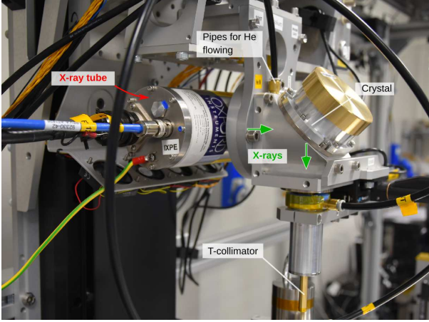
Figure 14: ICE polarized source during calibration of DU-FM2 with 2.70 keV polarized X-rays.
