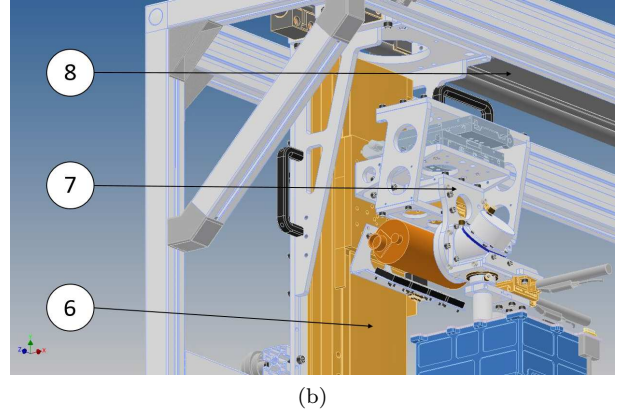
Figure 4: Detailed view of the tower supporting the DU (a) and of the source assembly (b). The items in the figures are the manual and motorized stages which allow one to align the X-ray beam and the DU (item 5). The beam is centered on the detector with two linear stages, item 3 and 4, and its angle of polarization with respect to the detector is changed with a third rotation stage (item 3). The detector tip/tilt is adjusted with a platform (item 1). The source height and tip/tilt are changed with item 6 and 7, respectively, and its position is slide with a manual stage (item 8).
