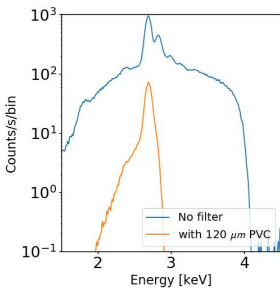
Figure 8: Example of the effect on the spectrum of direct X-ray tube with Rh anode with and without X-ray filter 120 \mu\text{m} thick to select the L\alpha fluorescence line.
