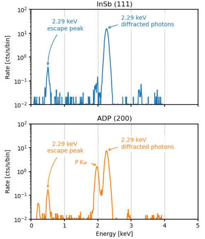
Figure 15: Comparison of spectra measured with the ICE test spectrometer of the polarized source at 2.29 keV with \text{InSb} (111) or \text{ADP} (200) crystals for the same X-ray tube settings. For the latter, the counting rate is lower and the presence of the fluorescence lines of phosphorus makes it difficult to estimate the polarization of the combined lines, which would be unresolved with the spectral resolution of the DU.
