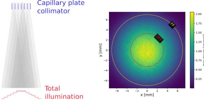
Figure 10: (Left) Illustration of the geometrical effect which causes a non-uniform illumination for fluorescence sources. (Right) Illumination measured for fluorescence source at 2.29 keV.
