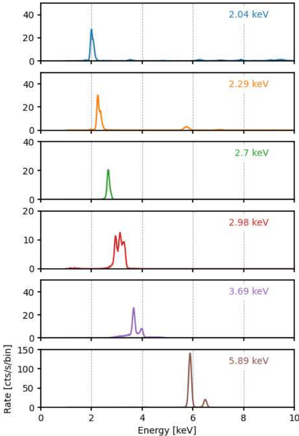
Figure 12: Spectra of unpolarized sources measured with the ICE test spectrometer. X-ray tube high-voltage setting and distance to detector are equivalent to those used for DU calibration.
