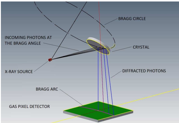
Figure 17: Geometry of Bragg diffraction for monochromatic photons.
