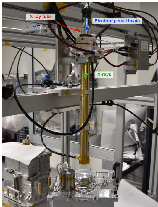
Figure 7: Geometry of head-on X-ray tube with Calcium anode.
