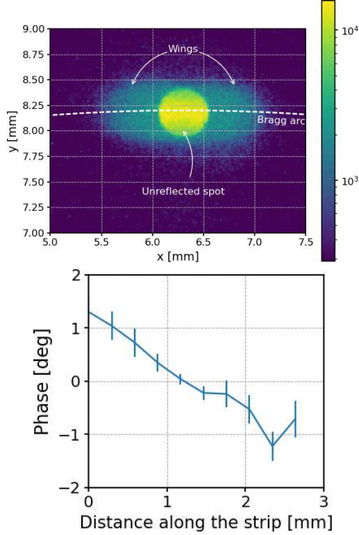
Figure 21: (Top panel) Image with the ICE test imager of the wings produced by reflection on inner walls of the capillary plates collimator at 2.70 keV. If the image is divided in vertical bins, the angle of polarization is not uniform but it remains tangent to the arc as expected.
