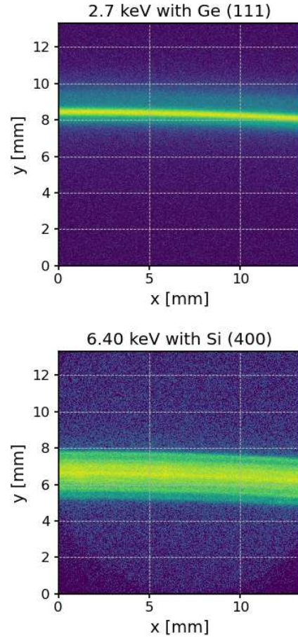
Figure 18: Image with the ICE test imager of the photons generated with the polarized source without collimators. In this condition, diffracted X-rays forms a “Bragg” arc on the detector, whose width depends on both the source and the crystal used. On the top there is the Bragg arc obtained with the X-ray tube with Rh anode and the Ge (111) crystal; on the bottom there is the Fe X-ray tube with Si (400) crystal.
