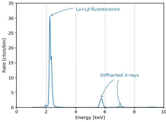
Figure 11: Spectrum of Zr fluorescence source measured with ICE test spectrometer.
