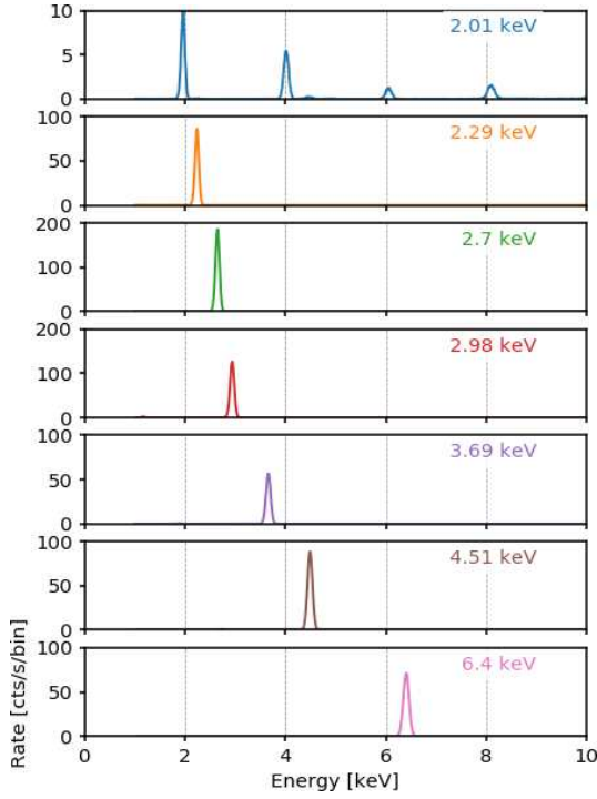
Figure 16: Spectra from polarized sources measured with the ICE test spectrometer.
