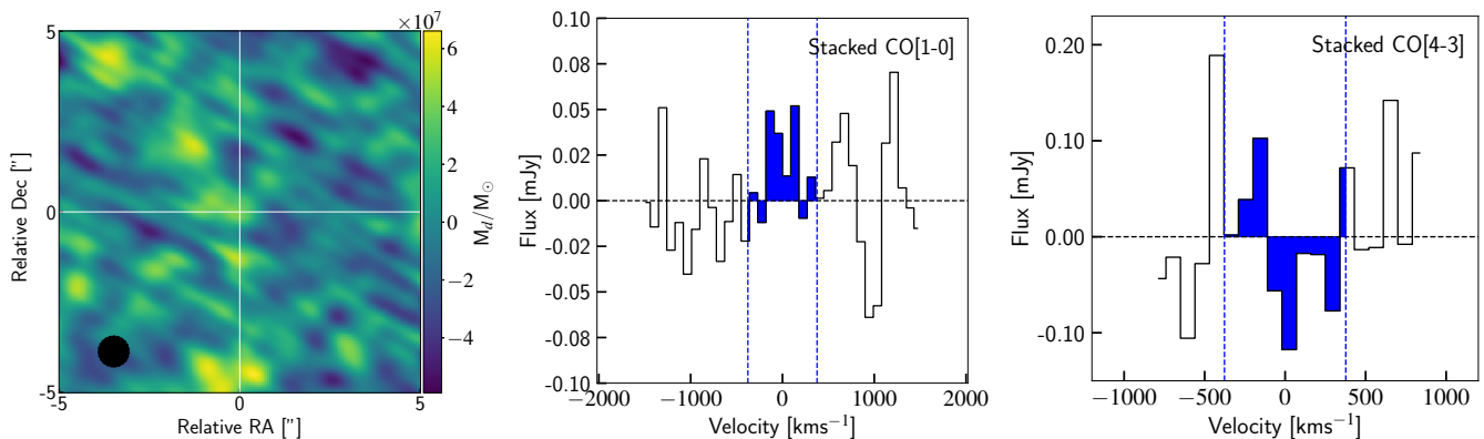
Figure 3. Left: stacked dust mass image for the five galaxies, created by combining the dust mass images from the 2mm data and 870 \mu m data, as described in the text. The image is centered on the position of the stacked galaxies, and the white crosshair highlights the position of the peak pixel, used to derive the upper limit on dust mass. The average of the circularised beams for the two continuum datasets is shown in the bottom left corner. Center: weighted-average stacked CO[1-0] spectrum of the five galaxies, binned into 90 km/s channels and shown against velocity relative to the expected position of the CO[1-0] line. The blue shading illustrates the average linewidth (containing 90% of the flux) of the galaxies, W_{90\%} = 753 \pm 22 \text{ km s}^{-1} , over which the stacked measurement was taken. Right: as for the center panel, but for the CO[4-3] spectral stack. The CO[4-3] spectrum covers a smaller velocity range than the CO[1-0] stack, as the spectral resolution was coarser in the sidebands used for continuum measurements.
