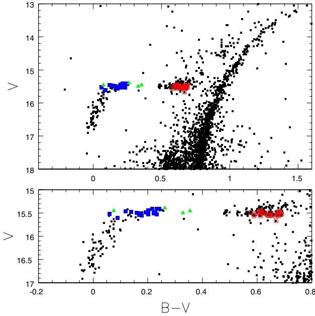
Fig. 1. Upper panel: (V, B - V) colour-magnitude diagram of NGC 6723 from Lee et al. (2014). Lower panel: blow-up of the HB region. Stars selected for observations are marked with large symbols: filled blue squares are BHB stars, open red squares are RHB stars, and filled green triangles are RR Lyrae variables.
