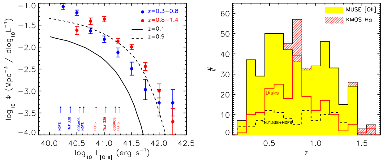
Figure 2. Left: [O II] luminosity function for the star-forming galaxies in our sample from the 18 MUSE IFU pointings. We split the sample into two redshift bins, z = 0.3 –0.8 and 0.8–1.4. The arrows on the plot denote luminosity limits for four of the fields in the MUSE sample (which span the complete range of depths). To baseline these results, we overlay the [O II] luminosity function at z = 0 from SDSS (Ciardullo et al. 2013) that shows that there is strong evolution in L_{\text{[O II]}^*} from z \sim 0 to z \sim 0.5 . This evolution is also seen in other [O II] surveys (e.g. Ly et al. 2007; Khostovan et al. 2015). Right: the redshift distribution of the [O II] and H \alpha emitters in our MUSE and KMOS samples. Our sample has a median redshift of z = 0.84 and a full redshift range of z = 0.28 –1.67. Since the MUSE observations have a wide range of exposure times, from 5.7 to 107.5 ks, we overlay the redshift distribution of the [O II] emitters in the two deepest fields, HDFS and TN J1338, to highlight that the highest redshift galaxies are not dominated by the deepest observations. We also overlay the redshift distribution of the galaxies classified as ‘rotationally supported’ (i.e. discs).
