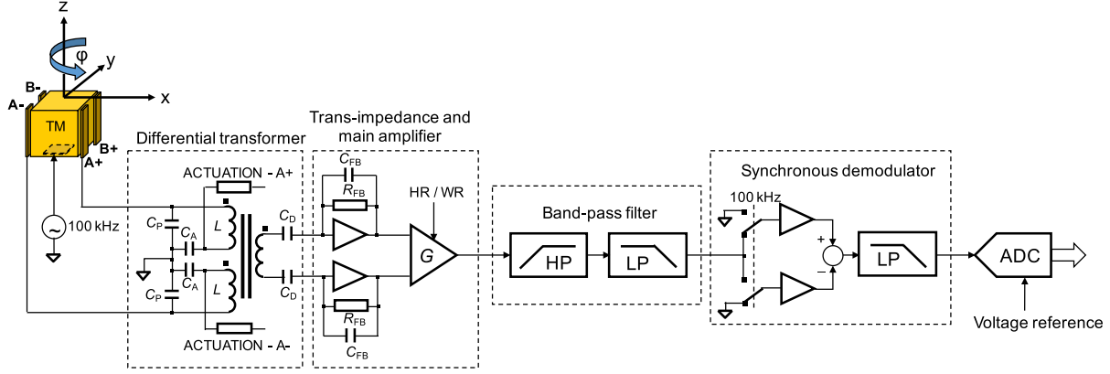
FIG. 1. A block diagram of the single TM sensing channel electronics along the x axis. Two pairs of electrodes ( A + / A - , B + / B - ) allow simultaneous measurement of the TM displacement and rotation, which is achieved by measurement of the gaps between the TM and the electrodes at opposing sides of the TM. For small TM displacements, the capacitance is proportional to the respective TM—electrode gap. The actuation circuit (one for each electrode) electrostatically applies forces and torques on the TM using the same electrodes. An ac injection bias (100 kHz) is injected on the TM. Differential currents are measured, amplified, and converted into an ac sensing voltage proportional to the TM motion. Sensing voltage is filtered at the ac injection frequency, and its amplitude is demodulated and finally converted into a digital value.
