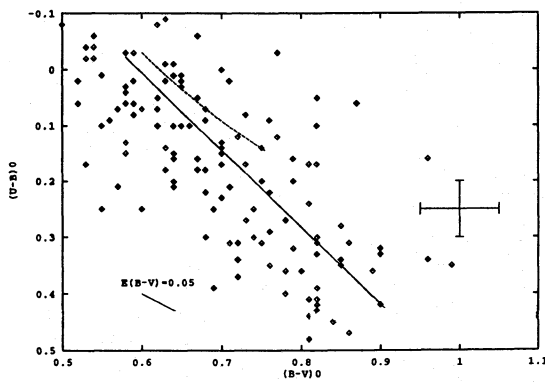
Fig. 9. Comparison between synthetic and observed indices for 141 M 31 GCs (Elson & Walterbos 1988) for an age of 15 Gyr on the plane U - B , B - V . Dotted and solid lines as in Fig. 5
