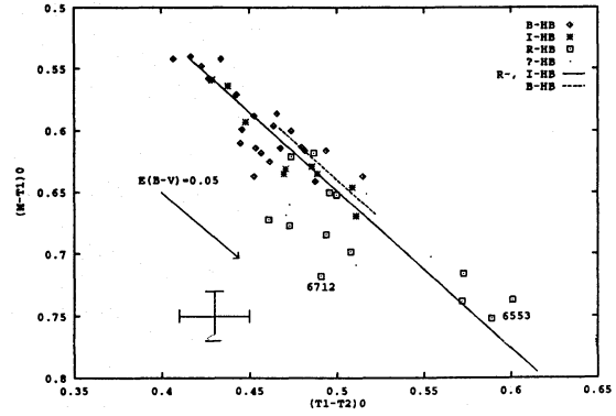
Fig. 7. Comparison between synthetic and observed indices for an age of 15 Gyr for 51 GGCs (Harris & Cantner 1977) on the plane M - T_1 , T_1 - T_2 of Washington Observatory system. Symbols as in Fig. 5
