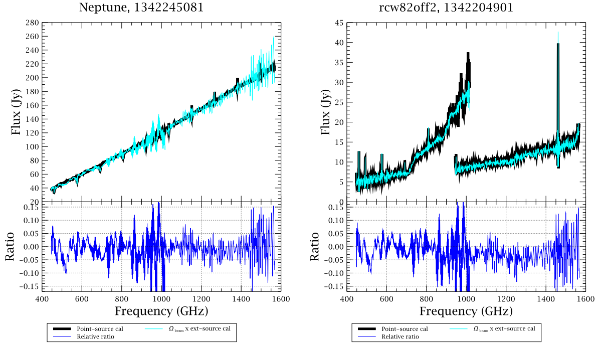
Figure 5. Left panel: comparison of Neptune pipeline derived point-source calibrated flux density S_S(\nu) in Jy (thick black line) with the flux density derived from the extended-source calibrated intensity S'_S = \eta_{\text{diff}} \times I'_S(\nu) \times \Omega_{\text{beam}} (cyan), i.e. Equation 11. The relative ratio of S'_S/S_S is shown in the bottom panel. The overall agreement, in the less noisy parts of the two bands, is within 5%. Right panel: the same comparison for a fully extended source.
