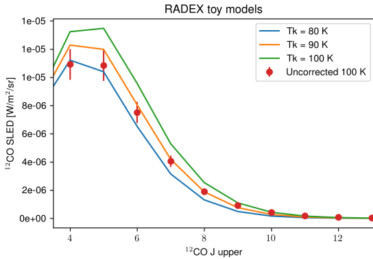
Figure 6. ^{12}\text{CO} spectral line energy distribution model from RADEX (van der Tak et al. 2007) for an emitting region, assuming n(\text{H}_2) = 6.3 \times 10^3 \text{ cm}^{-3} , column density of 10^{16} \text{ cm}^{-2} and kinetic temperatures of 100 K (green curve), 90 K (orange) and 80 K (blue). The 100 K SLED is multiplied by \eta_{\text{ff}} and the new uncorrected SLED is shown with red points with error bars assuming a conservative 10% uncertainty in line flux measurements.
