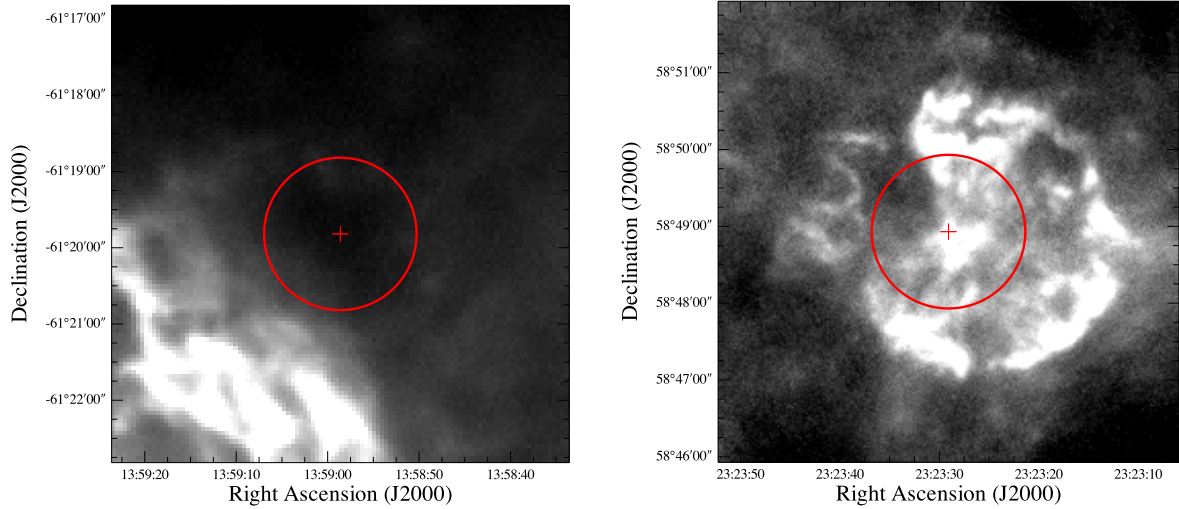
Figure 1. (Left) Spatially flat extended source, RCW82off2 (see Table 1), with greyscale image corresponding to the PACS 70 \mu\text{m} map and the 1' radius unvignetted FTS field of view shown as a red circle. The centre of the FTS field is marked with a '+' sign. Note that the region appears as dark due to the very bright nearby RCW82; the peak surface brightness within the FTS footprint at 250 \mu\text{m} is more than 400 MJy/sr. (Right) Cas A – a supernova remnant shown with 70 \mu\text{m} PACS data that was rejected because of its complex morphology although \Delta g_{\text{max}} = 0.07 and \sigma_I = 0.07 .
