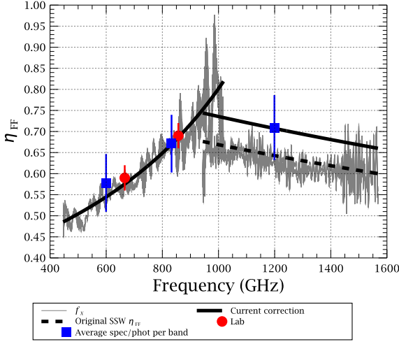
Figure 3. Averaged ratios of the synthetic photometry versus the results from photometer maps for all 24 flat sources (filled blue squares), together with the far-field feedhorn efficiency (black lines, see Equation 8) and the laboratory measurements from Chattopadhyay et al. (2003) (filled red circles). The dashed line is the original \eta_{\text{FF}} for SSW as presented in Wu et al. (2013). The grey curves are the ratios f_X = \eta_{\text{diff}} I_S \Omega_{\text{beam}} / S_S for all of the 24 flat sources (see section 4).
