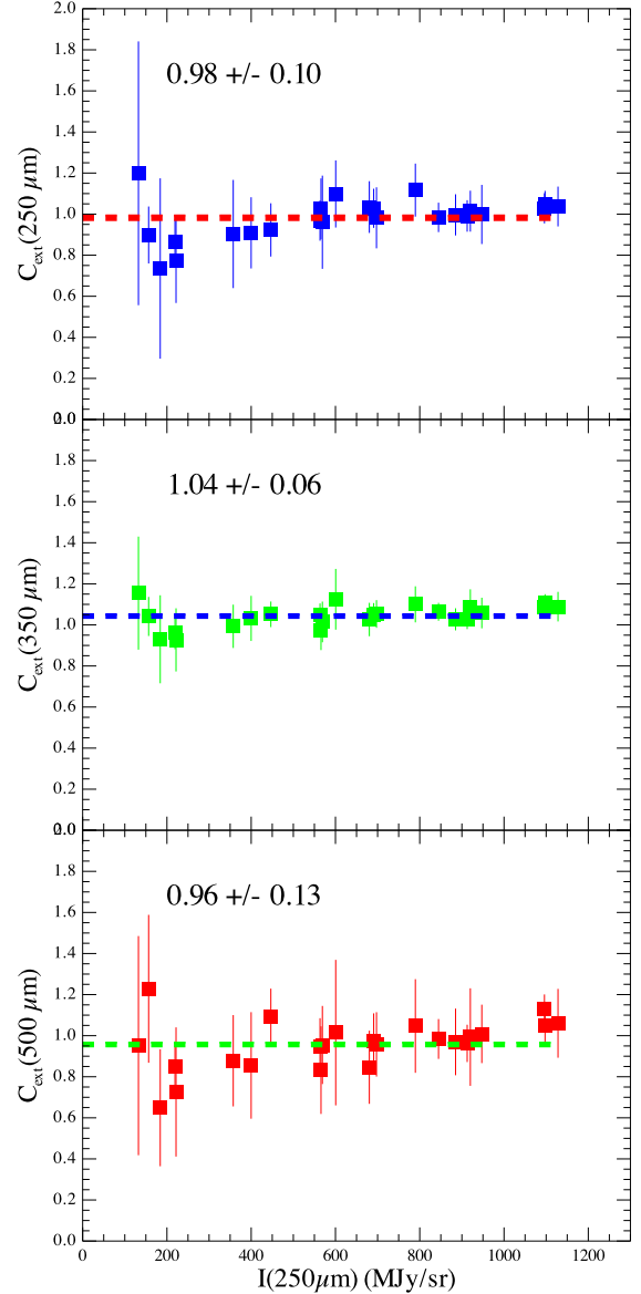
Figure 4. C_{\text{ext}}(\nu_0) = I_{\text{phot}}(\nu_0)/I_{\text{spec}}(\nu_0) as a function of \bar{I}_{250\mu\text{m}} at 250 \mu\text{m} (top), at 350 \mu\text{m} (middle) and 500 \mu\text{m} (bottom) for the 24 flat sources. The mean (shown as a dashed line) and the standard deviation for each band are annotated in each panel: from top to bottom, 250, 350 and 500 \mu\text{m} .
