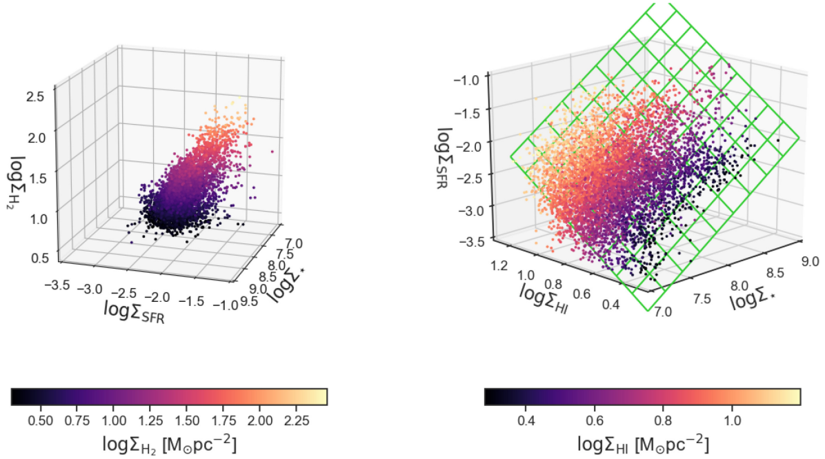
Figure 6. Left-hand panel: Distribution of the regions having an estimate of \Sigma_{\text{H}_2} above the sensitivity limit in the \log \Sigma_* – \log \Sigma_{\text{SFR}} – \log \Sigma_{\text{H}_2} plane. Each point is colour coded as a function of \log \Sigma_{\text{H}_2} . Four projections of this space at different azimuthal angles are shown in Fig. A1. Right-hand panel: Distribution of the regions having an estimate of \Sigma_{\text{H}_1} above the sensitivity limit in the \log \Sigma_* – \log \Sigma_{\text{SFR}} – \log \Sigma_{\text{H}_1} plane. Each point is colour coded as a function of \log \Sigma_{\text{H}_1} . The best-fitting plane is indicated by the green grid. Four projections of this plane, described by equation (7), at different azimuthal angles are shown in Fig. A2.
