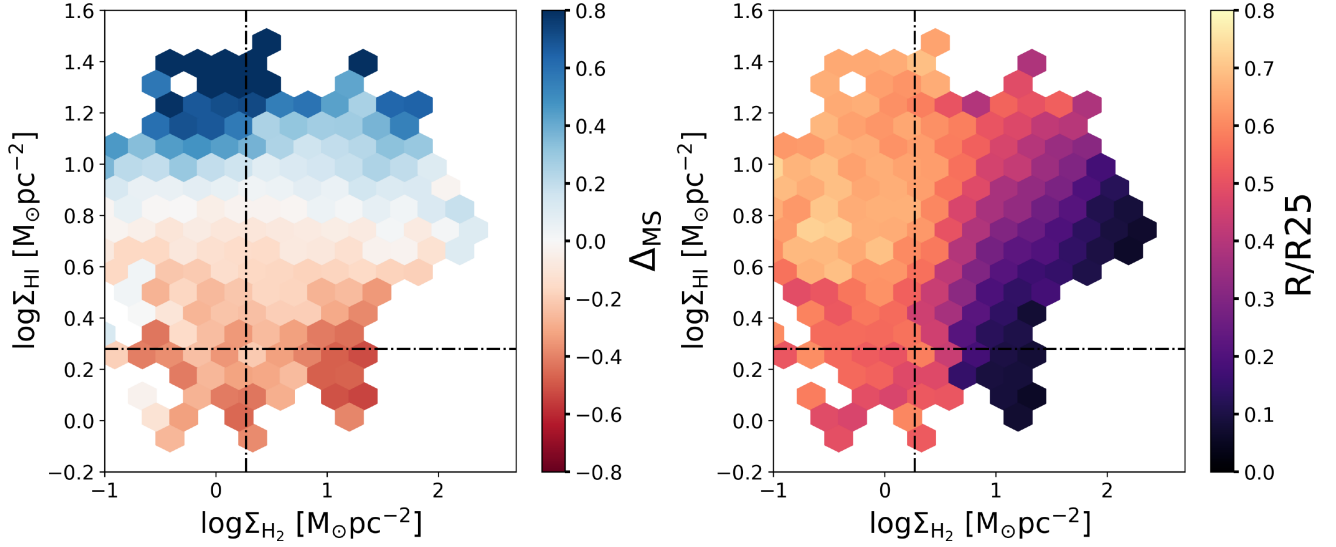
Figure 7. The \log \Sigma_{\text{H}_2} – \log \Sigma_{\text{H I}} plane, colour coded as a function of \Delta_{\text{MS}} (left-hand panel) and R/R_{25} (right-hand panel). Sensitivity limits are marked with dot–dashed lines.
