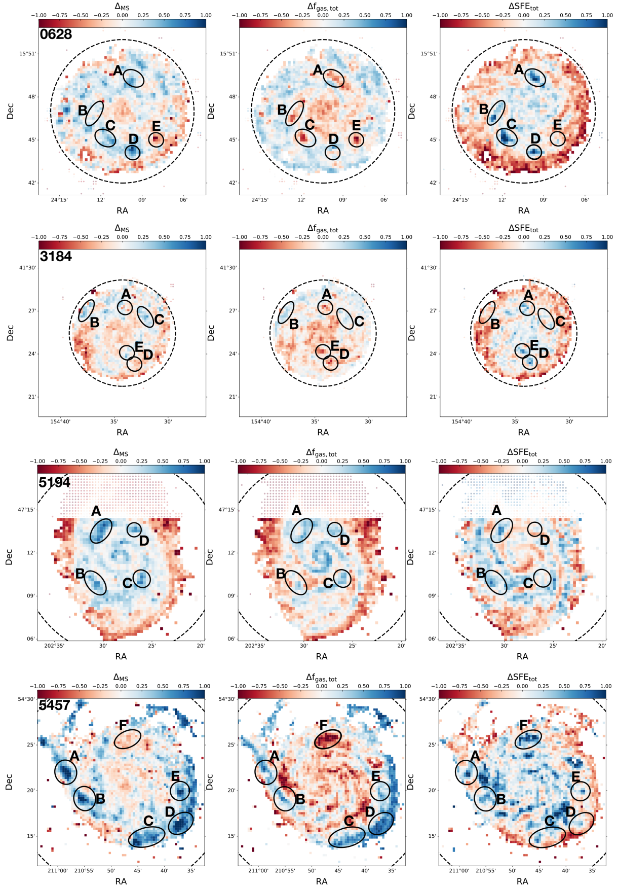
Figure B1. \Delta_{\text{MS}} (left), \Delta f_{\text{gas,tot}} (centre), and \Delta \text{SFE}_{\text{tot}} (right) maps of (from top to bottom) NGC 0628, NGC 3184, NGC 5194, and NGC 5457. The highlighted regions are discussed more in detail in the text.
