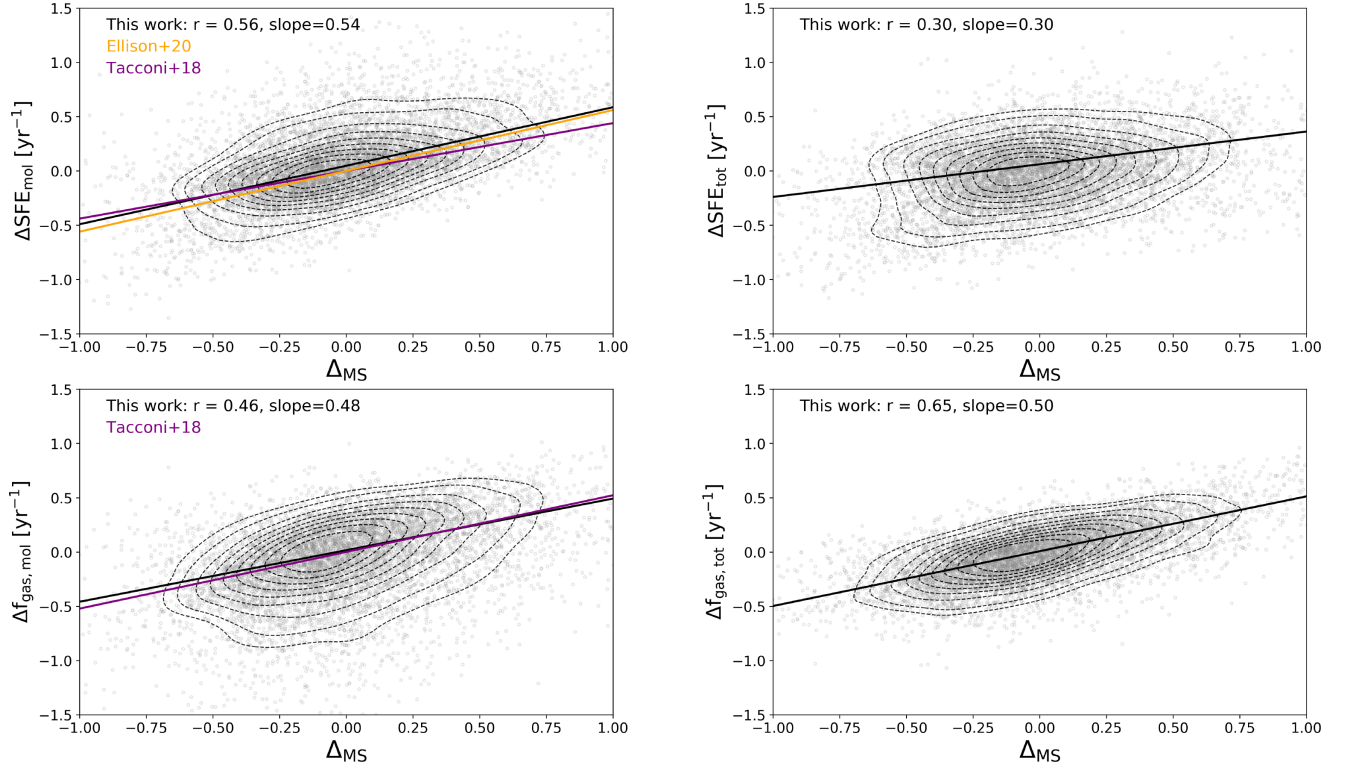
Figure 10. Distributions of regions in the \Delta_{\text{SFE, mol}}-\Delta_{\text{MS}} plane (top left-hand panel), in the \Delta_{\text{SFE, tot}}-\Delta_{\text{MS}} plane (top right-hand panel), \Delta_{f_{\text{gas, mol}}}-\Delta_{\text{MS}} plane (bottom left-hand panel), and \Delta_{f_{\text{gas, tot}}}-\Delta_{\text{MS}} (bottom right-hand panel). The best-fitting relations of this work are shown as a black solid line. The best-fitting slope and the Pearson correlation coefficient are written each panel. In the left-hand panels, we show relations of Tacconi et al. (2018) in purple, and the one of Ellison et al. (2020a) in orange.
