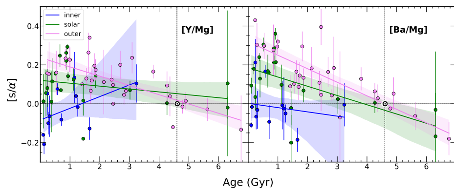
Figure 3. [s/\alpha] versus age in three Galactocentric bins (outer disc in pink, R_{GC} > 9 kpc; solar neighbourhood in green, 7 \leq R_{GC} \leq 9 kpc; inner disc in blue, R_{GC} < 9 kpc). The curves are the weighted linear fits to the data. In the left-hand panel we show [Y/Mg] versus ages, and in the right-hand panel [Ba/Mg] versus age. The data of individual clusters (abundance ratios are the mean values of the clusters members, while ages are from Cantat-Gaudin et al. [13], derived from Gaia DR2 data) are represented by filled circles, in the same colours as the corresponding fits. The shaded areas indicate the confidence intervals of the fits.
