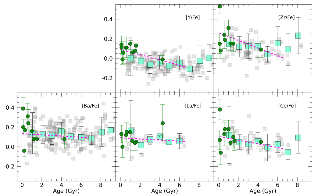
Figure 1. Abundance ratios [El/Fe] vs. age for the thin-disc stars (binned results, bin 0.1 dex wide—cyan squares, and individual stars—grey squares) and the open clusters located in the solar neighbourhood (green circles). The magenta dashed lines are the weighted linear fits to the cumulative sample of solar neighbourhood clusters and thin-disc field stars for stellar ages <8 Gyr (figure adapted from [29]).
