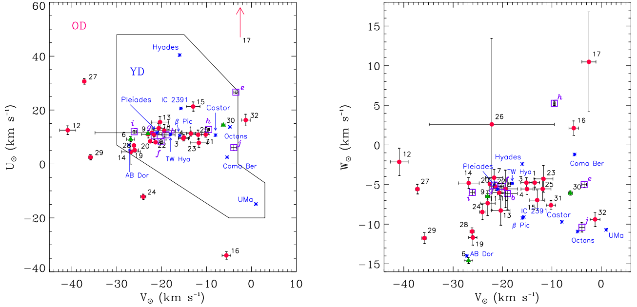
Fig. 10. ( V_{\odot} , U_{\odot} ) (left panel) and ( V_{\odot} , W_{\odot} ) (right panel) diagrams for PMS-like sources and two lithium-rich giants discussed in the paper. The symbols are as in Fig. 5 and the labels are as in Table 3. The average velocity components (blue asterisks) of some young SKGs and the locus of the YD population (Eggen 1996) are also indicated in the ( V_{\odot} , U_{\odot} ) plane. The position of the source #17 ( V_{\odot} = -2.5 \text{ km s}^{-1} , U_{\odot} = 83.5 \text{ km s}^{-1} ) is out of the scale of the plot, as indicated by the red arrow.
