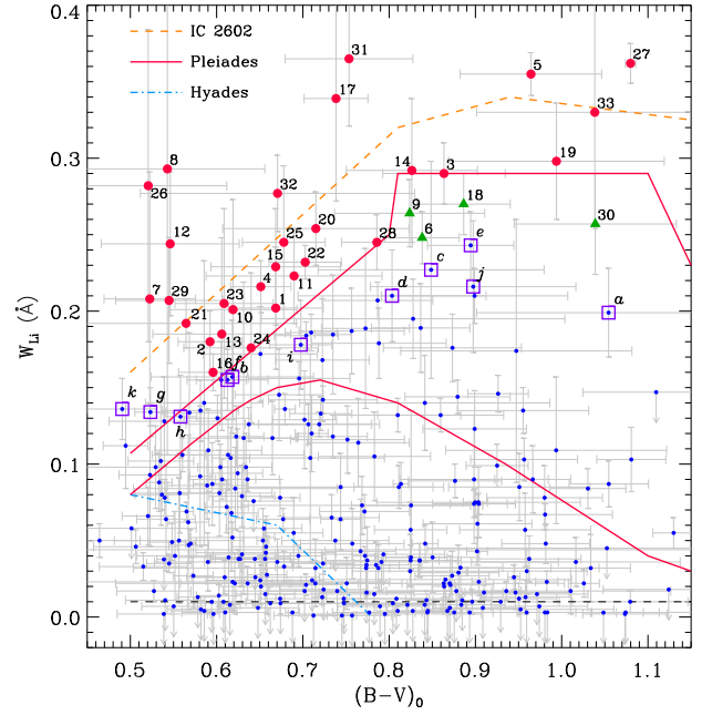
Fig. 5. Equivalent width of the Li I \lambda 6707.8 line ( W_{\text{Li}} ) plotted as a function of the dereddened Johnson (B - V)_0 color index for the single or SB1 stars in our sample (Table A.4). The lines show the upper boundaries for Hyades (blue dash-dotted), Pleiades (red solid for both lower and upper boundary), and IC 2602 (orange dashed) clusters. The black dashed line indicates the lower limit for positive detection of the Li I \lambda 6707.8 line estimated by us ( 10 \text{ m}\text{\AA} ). Twenty-nine stars (red big dots) show lithium equivalent width in excess with respect to the most lithium rich Pleiades stars and 10 of the stars fall above the upper envelope of the PMS cluster IC 2602. Four stars (green triangles) have W_{\text{Li}} just below the Pleiades upper envelope. The open squares enclose another 11 very young objects selected on the basis of their lithium abundance (see text and Fig. 6). All the lithium-rich stars are labeled according to Table 3.
