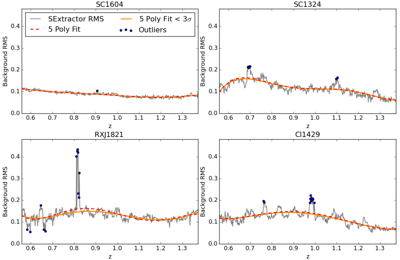
Figure 8. The background RMS as a function of redshift in four fields, SC1604, SC1324, RXJ1821, and CI1429. The gray lines are the background RMS as calculated by SExtractor. The dashed red line represents a fifth order polynomial fit without outlier rejection. The solid orange line represents a fifth order polynomial fit with iterative outlier rejection at above 3\sigma , based on the RMS of the preceding polynomial fit. The difference between the two fits with and without outlier rejection is largely minimal outside of areas with large peaks in the background RMS values. SC1604 is a very large field with deep imaging and shows a very flat RMS curve while CI1429 sees a much more variation in its RMS as a function of redshift. SC1324 and RXJ1821 show noticeable peaks at redshifts of 0.7 and 0.8 respectively, which correspond to known large structures in each field.
