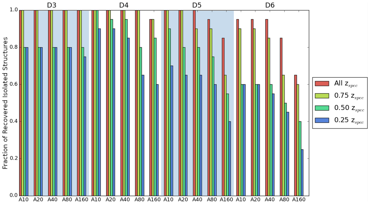
Figure 9. The recovered fraction of known structures in Table 2 based on different detection threshold ( D , in units of \sigma , given on the top axis) and minimum area ( A , in pixels, given on the bottom axis) parameters as well as fraction of available spectroscopic redshifts used in constructing the VMC maps. A known structures is considered successfully recovered if it lies within \Delta z = 0.02 of the nominal redshift and 1 Mpc of the nominal central coordinates. We found that a 4\sigma detection threshold was able to recover more structures at lower spectroscopic completeness.
