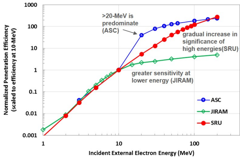
Figure 5. Comparison of the spectral sensitivities of the ASC, SRU, and JIRAM. The probabilities of omnidirectional high energy electrons to penetrate instrument shielding and create image noise events (“penetration efficiencies”) have been normalized to the value at 10-MeV for each instrument.
