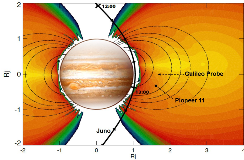
Figure 1. Juno’s “Perijove 1” trajectory through the inner magnetosphere on August 27, 2016. Times shown along the black trajectory curve are given in UTC with tick marks at 15 minute intervals. The spacecraft range was 1.06 Rj (4,147 km from the cloud tops) at closest approach; 12:50:44 UTC. The flyby provided a first look at territory not sampled by in-situ high energy particle instrumentation during past missions. Markers indicate the range of the Pioneer 11 spacecraft at its closest approach to the planet, and the path of the Galileo Probe into Jupiter’s atmosphere.
