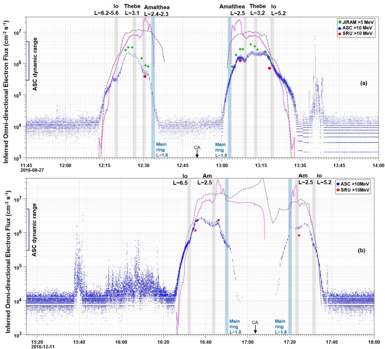
Figure 4. Omnidirectional fluxes of >5 \text{ MeV} and >10 \text{ MeV} electrons derived from penetrating particle count rates observed by the SRU, ASC, and JIRAM imagers along Juno's Perijove 1 (a) and Perijove 3 (b) trajectories. SRU and JIRAM measurements with count rates lower than the calibrated measurement range, or zero, have been omitted from the plot. ASC data have been corrected for electronic shutter time and filtered to remove samples affected by straylight. ASC data points at \sim 10^4 are due to a small star field dependent bias caused by dim stars reported amongst the count of penetrators (established with data collected during Juno's Cruise period outside of the Jovian magnetosphere). Grey bars show regions of L shell (calculated using the VIP4 magnetic field model [Connerney et al. , 1998] and the magnetodisc model of Connerney, Acuña, and Ness [1981]) associated with the orbits of several Jovian moons; blue bars mark L shells associated with the main Jovian ring; closest approach is marked "CA." Omnidirectional
