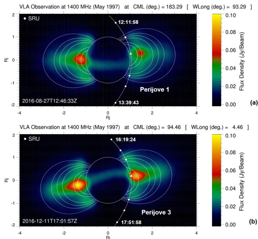
Figure 3. SRU image collection locations (white dots) along Juno's Perijove 1 (a) and Perijove 3 (b) science passes. Integrated flux density of synchrotron emission is shown ( \sim 21 cm, averaged over 20 degrees of longitude) for context. The synchrotron map projections (after Santos-Costa et al. [2014]) are given for the central meridian longitude corresponding to the System III West longitude of the spacecraft near the time of the magnetic equator crossing of each flyby (crossing times are shown in the lower left corners of the maps). Magnetic field lines are plotted for L=1.3, 1.5, 2, 2.25, 2.5, 3 and were calculated using the VIP4 magnetic field model [Connerney et al. , 1998]. SRU image collection was targeted to occur as Juno's trajectory grazed the inner edges of the high latitude lobes of the synchrotron region.
