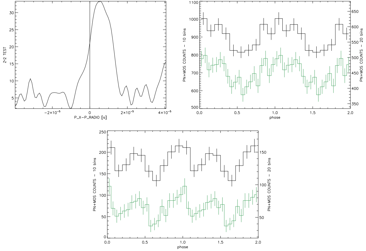
Fig. 3.— X-ray detection of PSR B. Top left: result of the Z^2_4 test distribution for 100 period search trials around PSR B’s radio ephemeris. Top right: background-subtracted PSR B profile for the 0.15-3.0 keV energy band obtained by folding the 2011 combined EPIC-MOS and EPIC-pn data (both light curves with 10 bins - in black - and 20 bins - in green - are displayed). Bottom: same as top right, but selecting the orbital phase interval \Delta\phi_{\text{orb}} = 0.58 - 0.78 .
