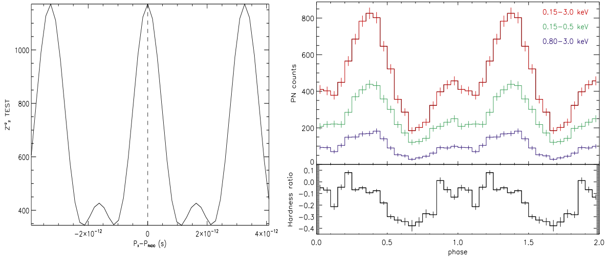
Fig. 1.— Left : Result of the pulsar spin period search trials around PSR A’s radio ephemeris solution. The most significant X-ray pulsed detection corresponds to a Z^2 -test value of \sim 1200 and is precisely aligned (within \sim 10^{-13} s) with the radio period indicated by the dashed vertical line. Top-right : Background subtracted light curve of PSR A for the energy band 0.15-3.0 keV (in red) and two sub-bands at low (0.15-0.5 keV, green) and high (0.8-3.0 keV, blue) energies, resulting from epoch folding of all available EPIC-pn data (2006+2011). Bottom-right : Phase-resolved hardness ratio between the hard (0.8 - 3.0 keV) and soft (0.15 - 0.3 keV) energy bands.
