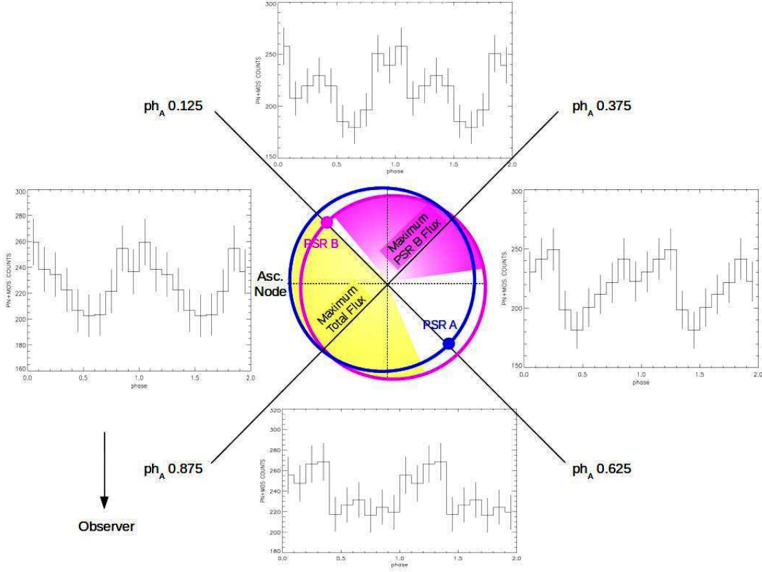
Fig. 4.— Central panel: scheme of the orbital configuration of PSR J0737–3039 in 2011 subdivided in four orbital phase intervals containing conjunctions ([0.125,0.375] - [0.625,0.875]) and quadratures ([0.875,0.125] - [0.375,0.625]). The yellow shaded region corresponds to the maximum of the total X-ray flux from the system (see §5 and Fig. 5), while the pink area indicates the maximum of the PSR B pulsed flux (both shaded regions highlight the phase intervals where PSR B is passing). The ph_A label in the figure highlights that phase 0 is referred to the PSR A ascending node. The four plots displayed around the scheme show the PSR B (background subtracted) pulse profile obtained by folding the 2011 EPIC-MOS and EPIC-pn counts belonging to the above mentioned orbital phases for the 0.15–3.0 keV energy band.
