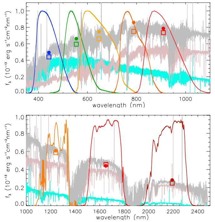
Fig. 10. X-shooter flux-calibrated spectrum of CVSO 104 A (pink line), CVSO 104 B (cyan line), and the sum of the two (grey line) in the visual (top panel) and NIR region (bottom panel). The contemporaneous photometry obtained from OACT in the BVR_cI_{c'} bands and the 2MASS JHK_s photometry are displayed with colored dots. The filter bandpasses and the synthetic photometry (open squares) obtained integrating the combined spectrum (A+B) over these bandpasses are overlaid with the same color as the photometric points.
