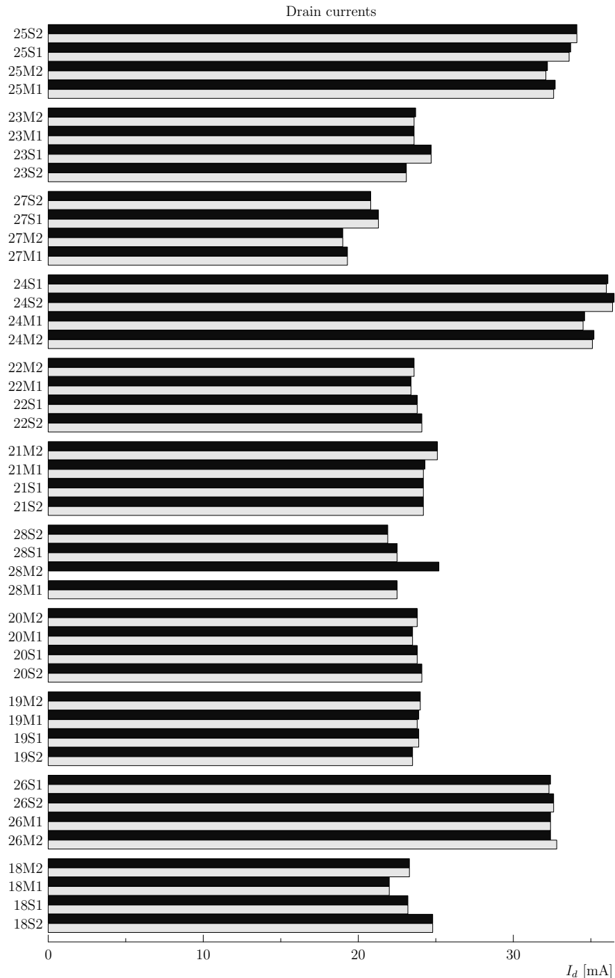
Figure 2: Comparison between the drain currents measured during the pre-cooling WFT (light bars) and the post-cooling WFT (dark bars). Data for #28 M2 was lost due to a TMH failure.
