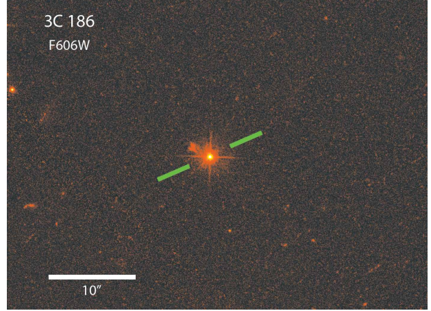
FIG. 34.— Central 35'' \times 50'' of the UVIS image of QSO 3C 186. The image has been rotated so that North is up and East to the left. Green lines are placed on either side of the target to help identify its location.
