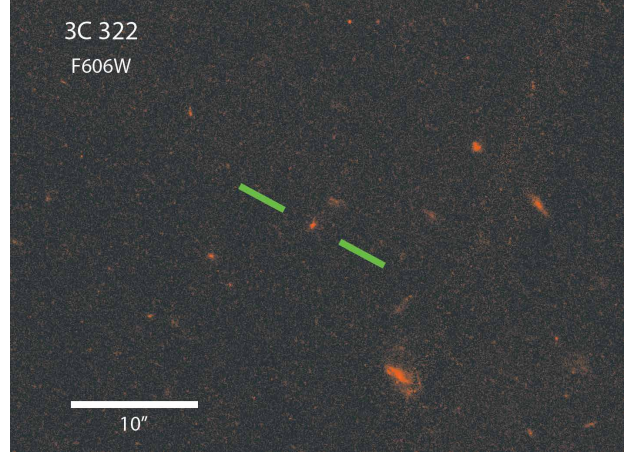
FIG. 22.— Central 35'' \times 50'' of the UVIS image of RG 3C 322. The image has been rotated so that North is up and East to the left. Green lines are placed on either side of the target to help identify its location.
