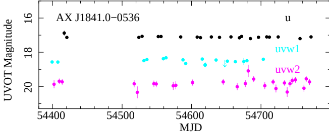
Figure 2: Swift /UVOT light curves of AX J1841.0–0536. Adapted from Romano et al. (2009b).
