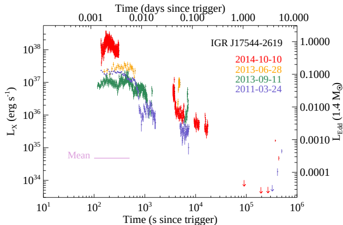
Figure 9: Bolometric X-ray luminosity light curves of the brightest outbursts recorded by Swift for IGR J17544–2619. The giant burst of 2014 October 10 is shown in red, and compared with previous bright outbursts from this source. The horizontal (pink) line marks the average level for this source, obtained from the two year monitoring campaign (Romano et al. 2011a, see Sect. 2.2), while the right-hand y-axis is the standard Eddington luminosity for spherical accretion of fully ionized hydrogen for a 1.4 M_{\odot} NS. Adapted from Romano et al. (2015).
