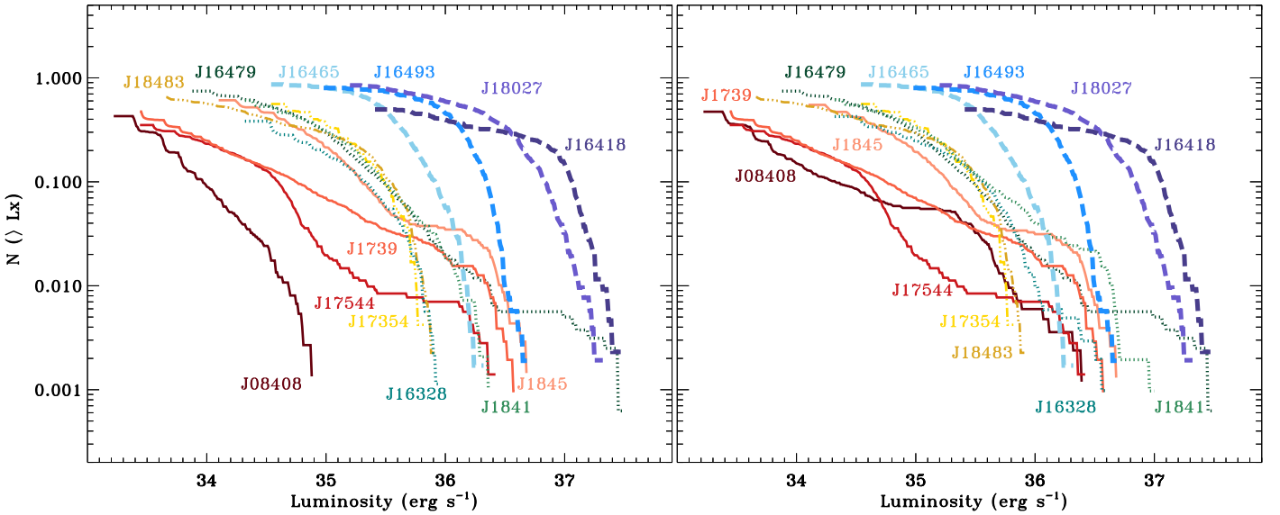
Figure 8: Cumulative luminosity distributions of the 2–10 keV luminosity drawn from the Swift /XRT light curves binned at 100 s. The classical SGXB IGR 18027–2016 is marked with a thick dashed line. Newly classified classical systems IGR J16465–4507, IGR J16418–4532, and IGR J16493–4348 are also marked with thick dashed lines. The intermediate SFXTs IGR J18483–0311 and IGR J17354–3255 are shown as dot-dashed lines. IGR J16328–4726, IGR J16479–4514, and AX J1841.0–0536 are shown as dotted lines, while the most extreme SFXTs (IGR J08408–4503, XTE J1739–302, IGR J17544–2619, and AX J1845.0–0433) are marked with solid lines. The data on IGR J16493–4348 and AX J1845.0–0433 are presented here for the first time, the rest are adapted from Bozzo et al. (2015) . Left: Only XRT data collected during the monitoring campaigns of all sources are used. Right: Same as for the left, but in this case we also considered one outburst for the sources IGR J08408–4503, IGR J16328–4726, AX J1841.0–0536, and AX J1845.0–0433 recorded by the XRT outside the corresponding monitoring campaigns.
