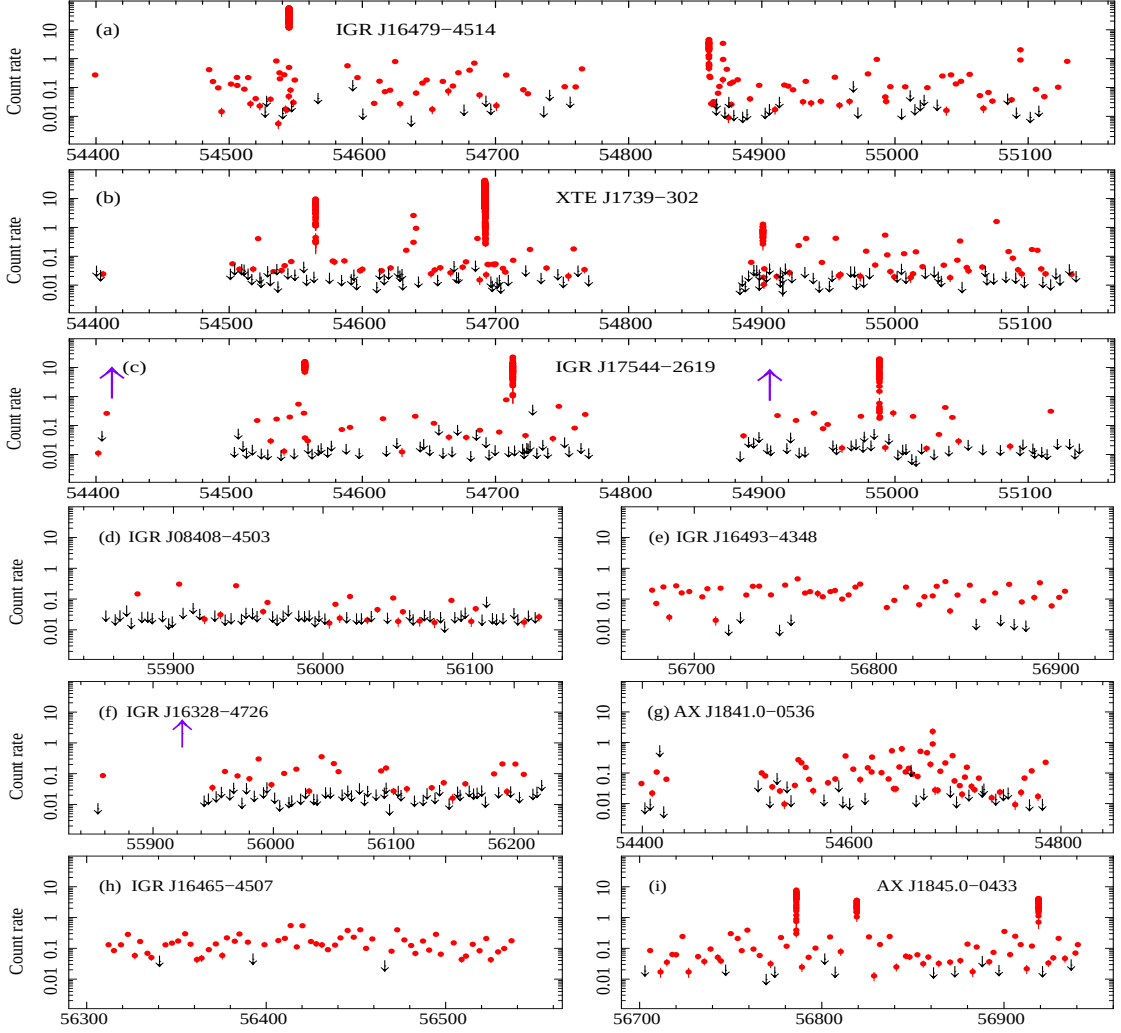
Figure 1: Swift /XRT (0.2–10 keV) long term light curves for the yearly monitoring sample . The x-axis is in MJD. The points refer to the average count rate measured for each observation except for outbursts, where the data were binned to include at least 20 counts \text{bin}^{-1} (to best represent the dynamic range). Red points are detections, black downward-pointing arrows are 3\text{-}\sigma upper limits. Violet upward-pointing arrows mark bright outbursts detected by BAT (and not simultaneously followed by XRT), or by MAXI (for AX J1841.0–0536). The data on IGR J16493–4348 (panel e) and AX J1845.0–0433 (panel i) are presented here for the first time. The remainder of the data are adapted from papers listed in Table 1 (Col. 17).
