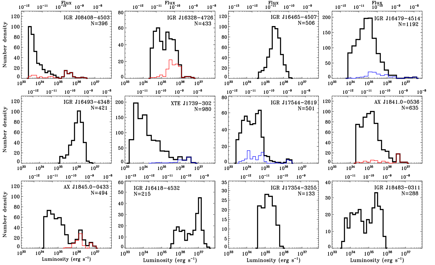
Figure 5: Differential distributions of the 2–10 keV luminosity (lower axis) and flux (unabsorbed, upper axis) drawn from the Swift /XRT light curves binned at 100 s. N is the sample size. The thick black lines represent the data collected during the monitoring campaigns (see Table 1, Col 4 and 5 for the campaign dates). The thin blue histograms show the part of the data collected as outburst observations during the campaign, thus including both the initial bright flare and the follow-up observations (see Sect. 3). The thin red histograms show outburst observations collected outside of the monitoring campaign (one outburst per source). The data on IGR J16493–4348 and AX J1845.0–0433 are presented here for the first time, the rest are adapted from Romano et al. (2014a).
