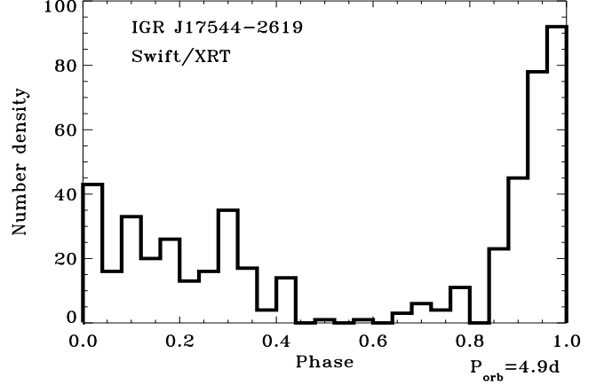
Figure 6: Distribution of the XRT detections (count rates) of IGR J17544–2619 (0.2–10 keV) folded at the orbital period, based on the most recent outburst ephemeris for this source ( P = 4.92693 \pm 0.00036 d, periastron at MJD 53732.65 \pm 0.23 ; Smith 2014).
