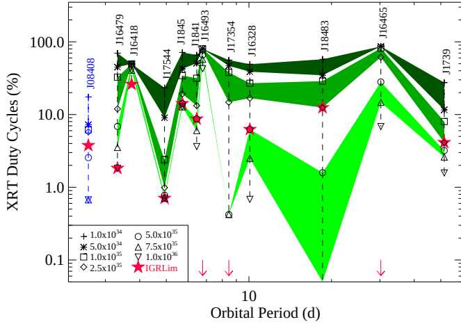
Figure 7: The XRT duty cycle (2–10 keV) as a function of orbital period and for a range of 2–10 keV luminosities (see legend, in units of \text{erg s}^{-1} ) in black. Only points above 0.1 % are shown. Since the period of J08408 is currently unknown (see Table 1 Col. 2 for the values adopted for the rest of the sample), we arbitrarily place it at an orbital period of about two days and mark it in blue. The shaded areas mark the loci of the XRT duty cycle defined by contiguous luminosities. The red filled stars represent the XRT duty cycle at the INTEGRAL sensitivity for each object (the downward-pointing arrows are consistent with 0). The data on IGR J16493–4348 and AX J1845.0–0433 are presented here for the first time, the rest are adapted from Romano et al. (2014a).
