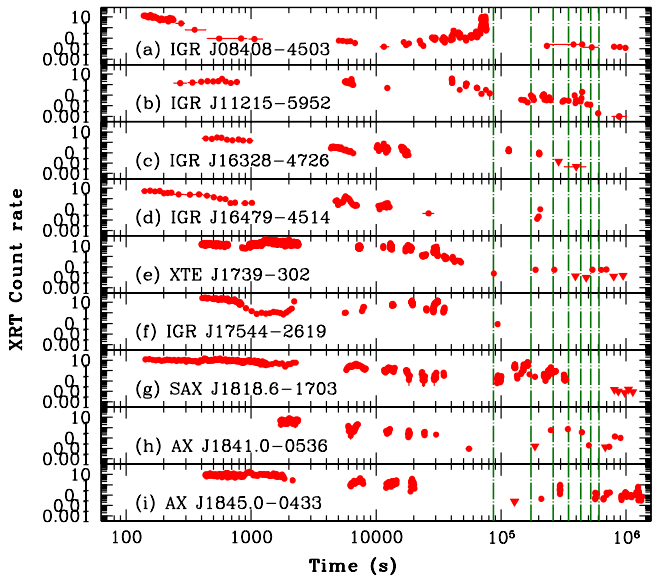
Figure 4: Swift /XRT light curves of the better followed-up outbursts of confirmed SFXTs, referred to their respective BAT triggers (except: IGR J11215–5952 is referred to MJD 54139.94). Points mark detections, triangles 3\sigma upper limits, vertical dashed lines mark daily intervals, up to a week. Data references: IGR J08408–4503 (2008-07-05, Romano et al. 2009a); IGR J11215–5952 (2007-02-09, Romano et al. 2007); IGR J16328–4726 (2009-06-10, Romano et al. 2013); IGR J16479–4514 (2005-08-30, Sidoli et al. 2008); XTE J1739–302 (2008-08-13, Sidoli et al. 2009a); IGR J17544–2619 (2010-03-04, Romano et al. 2011b); SAX J1818.6–1703 (2009-05-06, Sidoli et al. 2009b); AX J1841.0–0536 (2010-06-05, Romano et al. 2011b); AX J1845.0–0433 (2012-05-05, Romano et al. 2013). Adapted from Romano et al. (2013).
