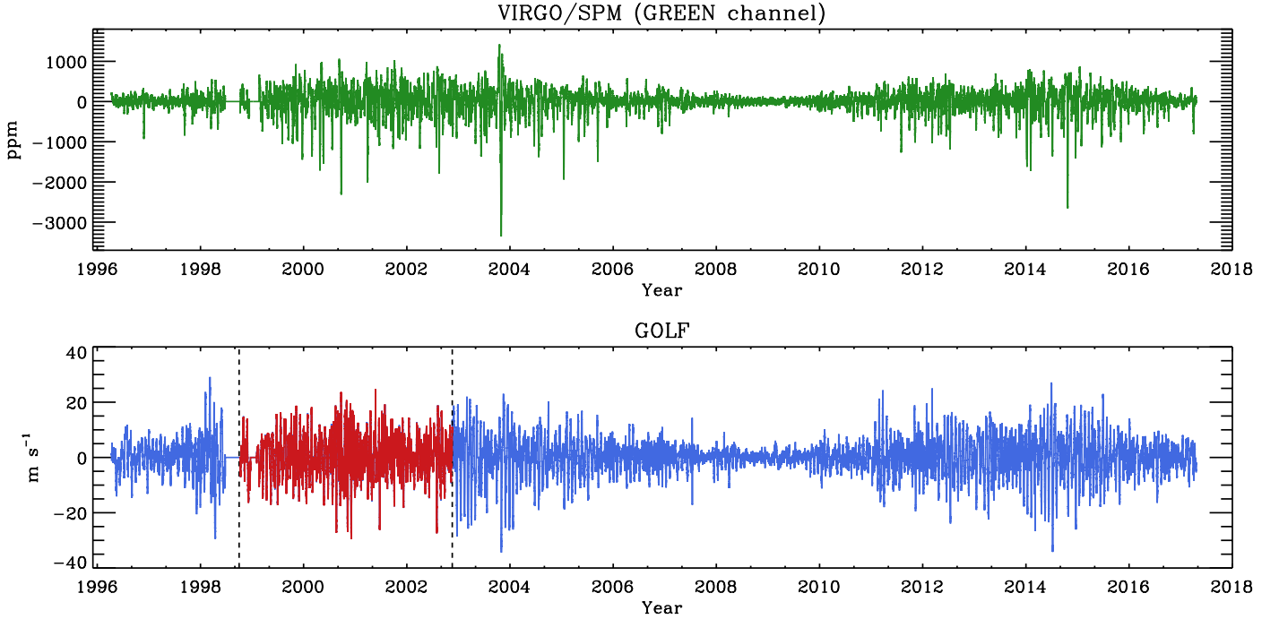
Fig. 1. Space-based observations of the Sun collected by the photometric VIRGO/SPM ( top panel , here the GREEN channel) and the radial velocity GOLF ( bottom panel ) instruments on board the SoHO satellite between 1996 April 11 and 2017 April 11. The missing data shown at zero between the years 1998 and 1999 correspond to the two temporary losses of SoHO. The GOLF red-wing period from mid-1998 to the end of 2002, denoted by the two vertical dashed lines, is represented in red (see Sect. 2).
