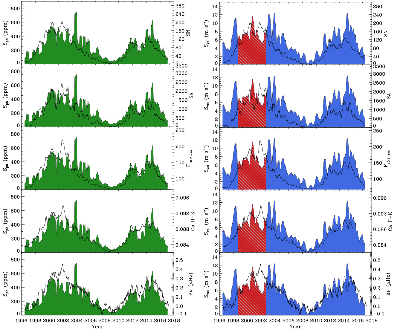
Fig. 3. Magnetic activity proxies S_{\text{ph, GREEN}} (in ppm) and S_{\text{vel}} (in \text{m s}^{-1} ) measured from the photometric VIRGO/SPM GREEN channel (GREEN filled, left panels ) and the radial velocity GOLF (BLUE filled, right panels ) observations as a function of time and compared to standard indices of solar activity (solid black lines). From top to bottom , the total sunspot number (SN), total sunspot area (SA), 10.7-cm radio flux ( F_{10.7\text{-cm}} ) in 10^{-22} \text{ s}^{-1} \text{ m}^{-2} \text{ Hz}^{-1} , Ca II K-line emission index in Å, and mean frequency shifts of the l = 0, 1 and 2 acoustic oscillations ( \Delta\nu ) in \mu\text{Hz} are shown. The red shaded areas in the right-hand panels represent the period when GOLF was observing in the red wing of the sodium line.
