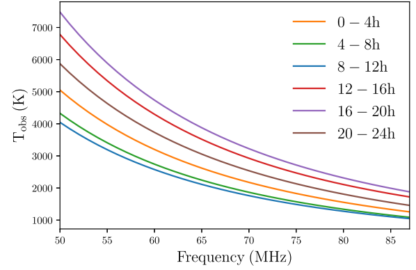
Figure 8. Simulated antenna temperature as seen through the LEDA beam as a function of frequency in the 50–87 MHz range. The different colours correspond to different 4 h LST bins.
