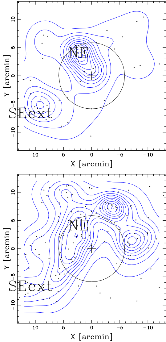
Fig. 12. Spatial distribution and isodensity contour maps of vsELGs (upper panel) and other ELGs (i.e., mELGs+sELGs, lower panel). The position of labels are those in Fig. 11 (lower right panel) to allow an easy comparison with that figure and highlight the concentration of vsELGs in the NE and SEext structures. The R_{200} region is indicated by the circle centered on the BCG.
