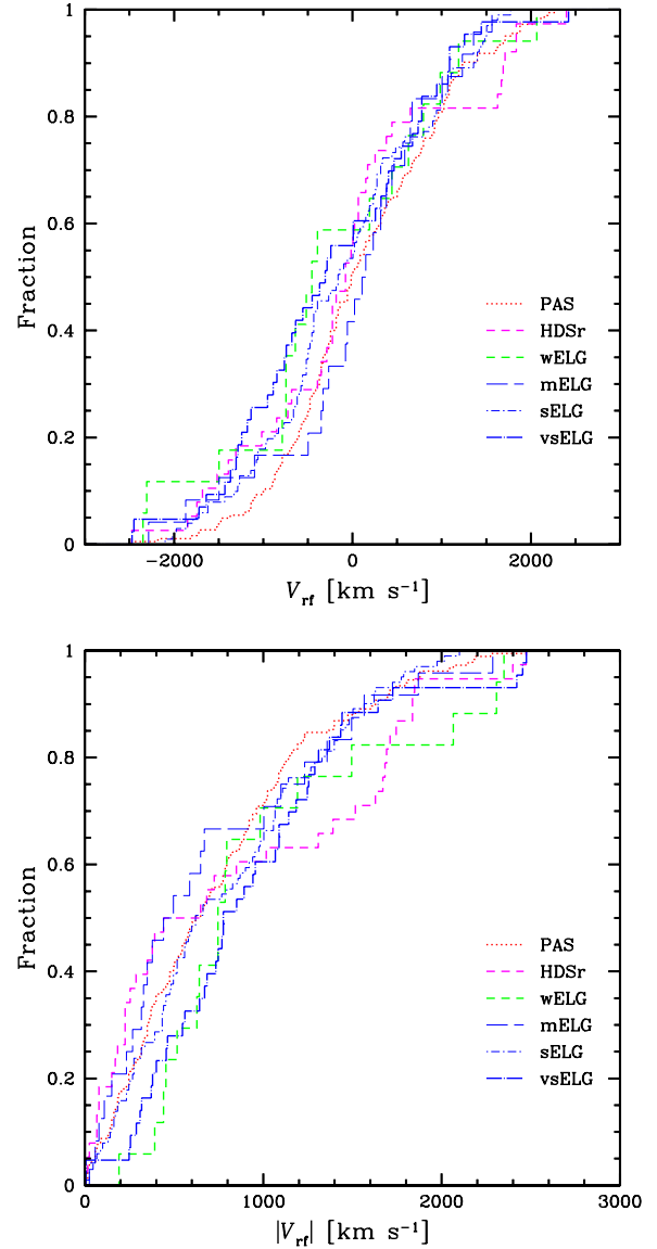
Fig. 6. Cumulative distributions of rest-frame LOS velocity V_{\text{rf}} and absolute V_{\text{rf}} of galaxies per spectral class ( upper and lower panels , respectively).
