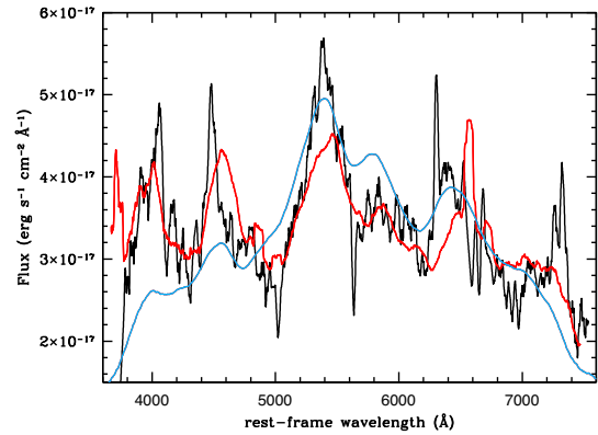
Figure 6. Spectrum of iPTF15dld of 2015 November 6 (black) dereddened with A_V = 0.085 compared with those of SN 1997ef (red) and SN 1998bw (blue) at comparable rest-frame phases. The spectrum of SN 1998bw was dereddened with A_V = 0.16 , while that of SN 1997ef needs no absorption correction. All spectra were smoothed with a boxcar of 50 \text{ \AA} . The absorption lines of SN 1998bw are significantly broader than those of iPTF15dld, while those of SN 1997ef represent a better match.
