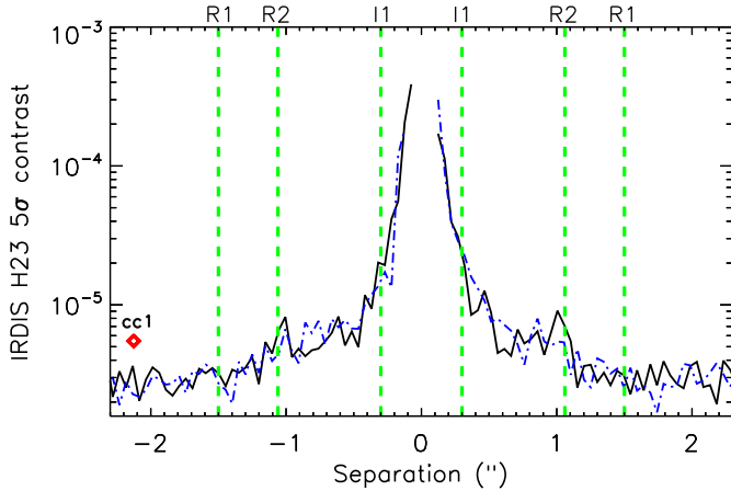
Fig. 11. 5\sigma contrast measured in the H23 TLOC1 reduction of May 15 2015, along PA = 146^\circ , parallel to the ellipse’s major axes (black solid line, negative is southeast); and PA = 56^\circ , the ellipse’s minor axes (blue dash-dotted line, negative is northeast). The vertical green dashed lines display the semi-major axes of R1, R2, and I1 as annotated above the top axis of the plot. The red diamond shows the measured signal of cc1 (which, we find, corresponds to 0.8 \pm 0.1 M_{\text{jup}} ). Notice that the actual location of cc1 does not coincide with either the minor or the major axes of the disk.
