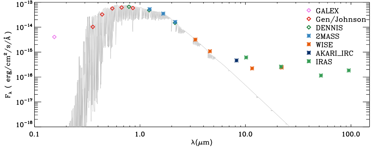
Fig. A.1. Spectral energy distributions (SED, see legend) and our best fit BT-NextGen model (grey solid line, T_{\text{eff}} = 4100 \text{ K} ) for RX J1615.
