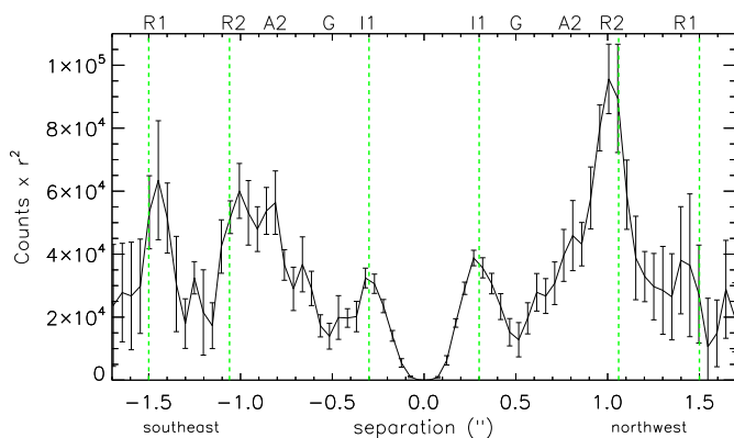
Fig. 7. Q_\phi intensity profile of r^2 scaled J -band image (Fig. 1c) along PA = 146.5°. The green dashed lines indicate the semi-major axes of the ellipses R1, R2 and I1. We note that although this profile is measured for a PA similar to those of the ellipses, the profile does include the star center, and therefore does not lie on the major axes of R1 and R2. This explains why the peaks of the rings lie at closer separations than their semi-major axes.
