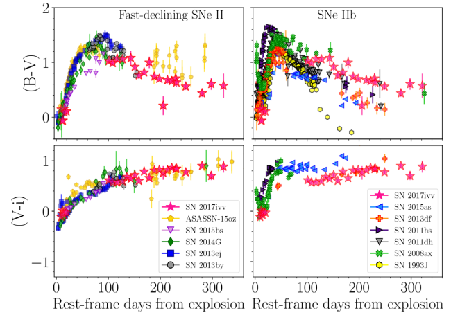
Figure 4. Colour evolution of SN 2017ivv compared to fast-declining SNe II (left-hand panels) and SNe I Ib (right-hand panels). See Section 4.1 for the references.
