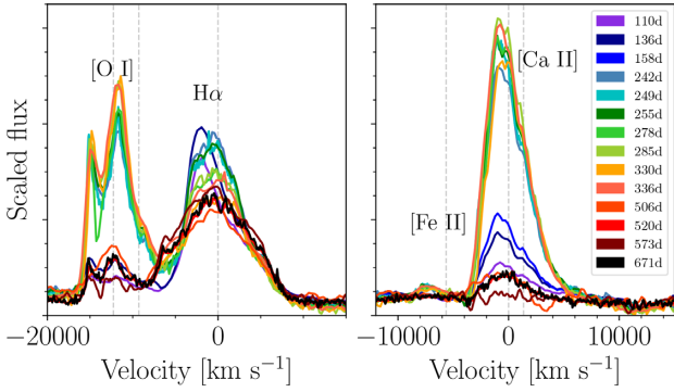
Figure 12. Observed profiles of SN 2017ivv in the nebular phase. Left-hand panel: [O I] \lambda\lambda 6300, 6364 and H\alpha emission lines. Right-hand panel: [Fe II] \lambda\lambda 7155, 7172 and [Ca II] \lambda\lambda 7291, 7324 emission lines. The phases are labelled on the right.
