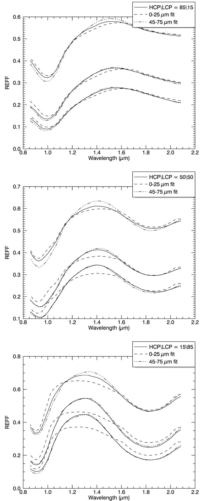
Fig. 8. HCP/LCP = 85/15 (top), 50/50 (middle), 15/85 (bottom) mixture fitting. In every plot, from top to bottom: 0–45 \mu\text{m} , 45–75 \mu\text{m} , and 75–125 \mu\text{m} grain size mixtures. Dashed lines and dot-dashed lines refer to model spectra synthesized using respectively endmembers with 0–25 \mu\text{m} or 45–75 \mu\text{m} .
