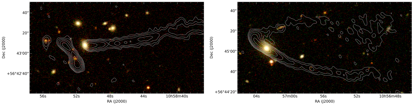
Figure 4. SDSS g , r , i optical images overlaid with GMRT contours at 610 MHz. The levels are [3, 6, 12, 24, 48, 96] \times \sigma where \sigma = 20 \mu\text{Jy beam}^{-1} . Left: the optical source associated with the HT GRG is the elliptical galaxy SDSS J105851.01+564308.5 at a redshift of z \approx 0.139 , within Abell 1132. The double source to the east of the HT is likely associated with the background galaxy SDSS J105852.18+564255.3 at a redshift of z \approx 0.496 . Right: the optical source associated with the WAT is the elliptical galaxy SDSS J105702.79+564503.1 at a redshift of z \approx 0.136 , within Abell 1132.
