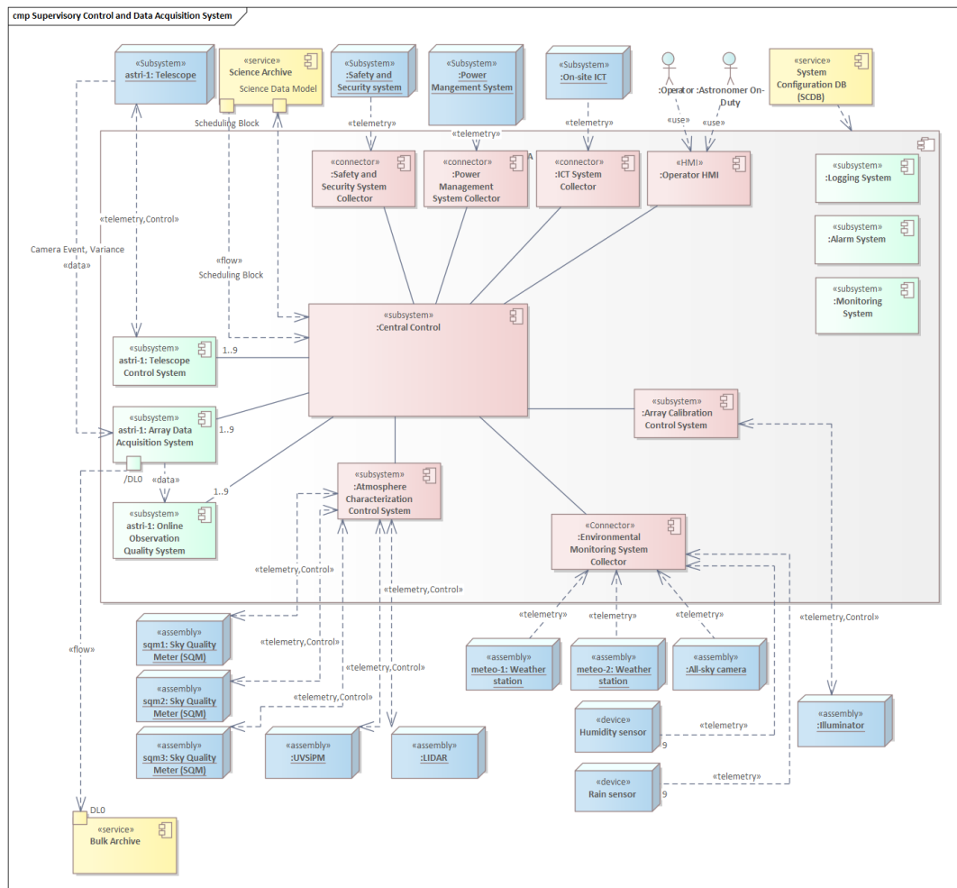
Figure 6. SCADA component diagram. Logging system acquires logs from all systems. Monitoring system acquires monitoring points from all assemblies and software systems. Alarm system receives alarms from assemblies. Only one telescope (and related subsystems) is shown, but there are nine independent chain of control, data acquisition and quality checks. Not all connections are shown, in particular the interconnections between Control Software/Collectors and Central Control are not shown and all connection between Alarm System, Monitoring System and Logging System are not shown. Red and green boxes are the SCADA system, where green boxes are under development by INAF team; blue boxes are the ASTRI Mini-Array assemblies; yellow boxes part of the Archive System. The << telemetry >> stereotype represents monitoring points, alarms, errors, logs, and status information, << data >> stereotype represents the data flow. The << control >> stereotype represents the control flow. DL0 is the raw data generated by scientific instruments.
