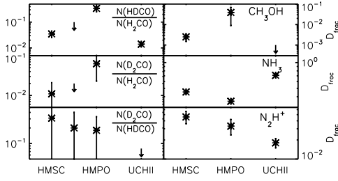
Fig. 1. Comparison of the average deuterated fraction of \text{H}_2\text{CO} , \text{HDCO} , \text{CH}_3\text{OH} , \text{NH}_3 , and \text{N}_2\text{H}^+ . The upper limit for G5.89-0.39 is not shown in the left middle panel, the value is <0.001 . Average values for \text{CH}_3\text{OH} , \text{NH}_3 , and \text{N}_2\text{H}^+ based on Fontani et al. (2015) are shown.
