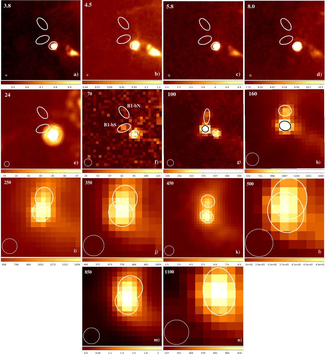
Fig. 1. Maps of 1'.5 \times 1'.5 of B1-bS and B1-bN at all wavelengths, with sizes and positions derived from the Gaussian fits. The FWHM of the respective instrumental beam is shown as a circle in the bottom-left corner of each respective panel. At \lambda \leq 100 \mu\text{m} , the source S295 is also visible. Colour bars are in Jy/beam for the SCUBA maps, and MJy/sr in all the others. In the Spitzer images, positions and sizes of the sources are copied from the 70 \mu\text{m} map. IRAC maps are in the top row, from left to right: a) 3.8 \mu\text{m} ; b) 4.5 \mu\text{m} ; c) 5.8 \mu\text{m} ; d) 8.0 \mu\text{m} . Second row: e) Spitzer 24 \mu\text{m} ; f) PACS 70 \mu\text{m} , B1-bN is not really detected and its flux corresponds to a 1\sigma rms point source; g) PACS 100 \mu\text{m} ; h) PACS 160 \mu\text{m} , S295 is no longer visible. Third row: i) SPIRE 250 \mu\text{m} ; j) SPIRE 350 \mu\text{m} ; k) SCUBA 450 \mu\text{m} , where the beam shown is 11'' , see Appendix A.2; l) SPIRE 500 \mu\text{m} . Bottom row: m) SCUBA 850 \mu\text{m} ; n) Bolocam 1.1 \text{ mm} , where only one source has been fitted.
