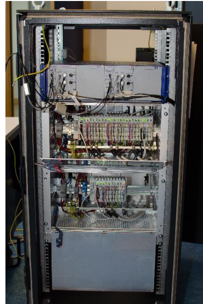
Figure 5: FEU #4 cabinet.
