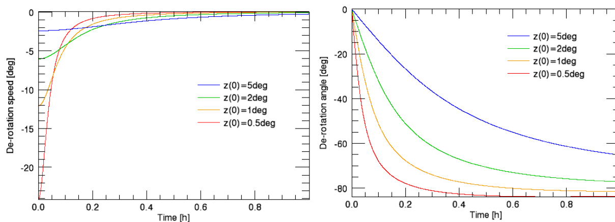
Figure 4 De-rotation speed and angle for object with different zenithal distance at transit.
