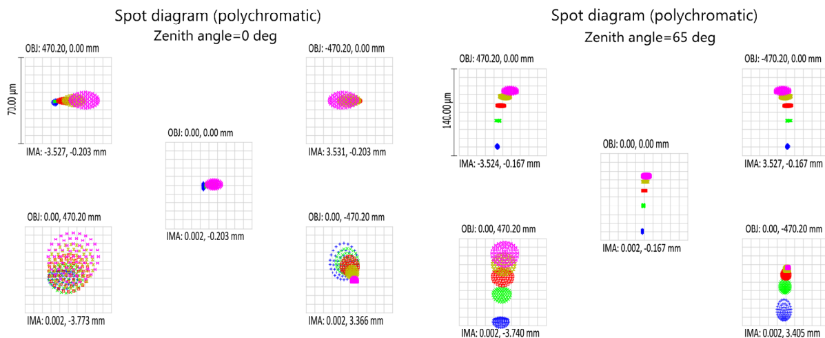
Figure 2 Spot diagram for the pupil image on the scientific detector (for the full bandwidth) when using the ADC to correct atmospheric dispersion at ZA=0deg (left) and ZA=65deg (right).
